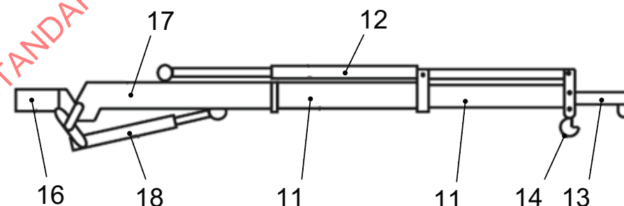
b) Loader crane with articulated boom
