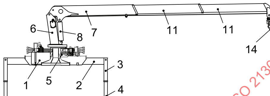
a) Loader crane with straight boom
