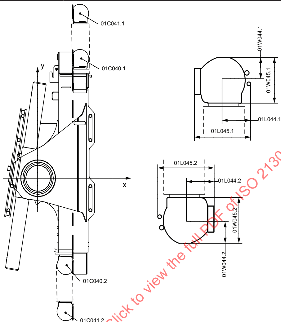
Example of coding of main stabilizers
