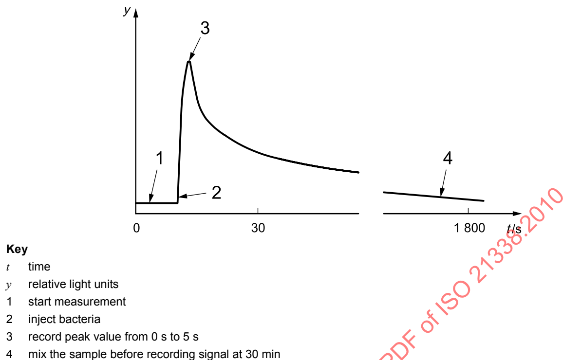
Figure 1 — Principal schematic protocol for the kinetic luminescent bacteria test
