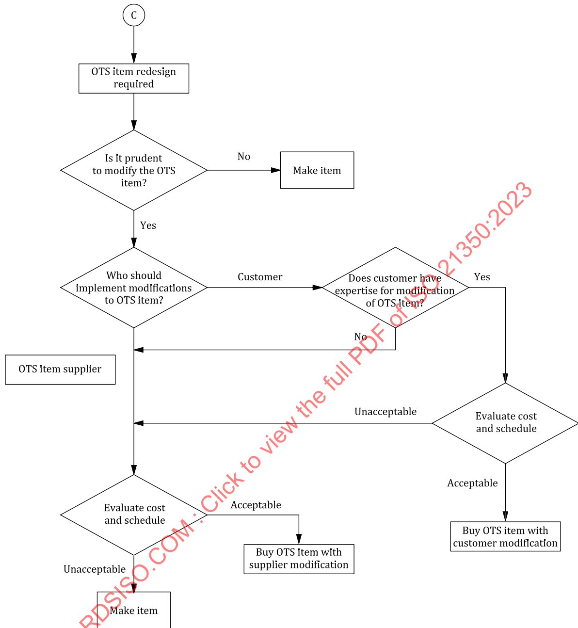
Figure A.1 — (3 of 3) Decision logic for OTS item utilization
