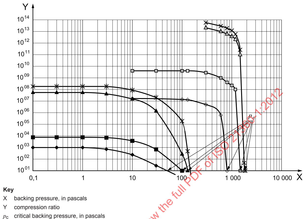
Figure 9 — Compression ratio curves of turbomolecular pumps
