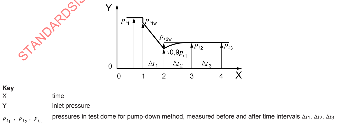
Figure 7 — Pressure versus time curve of pumping cycle for a volume flow rate measurement by the pump-down method
