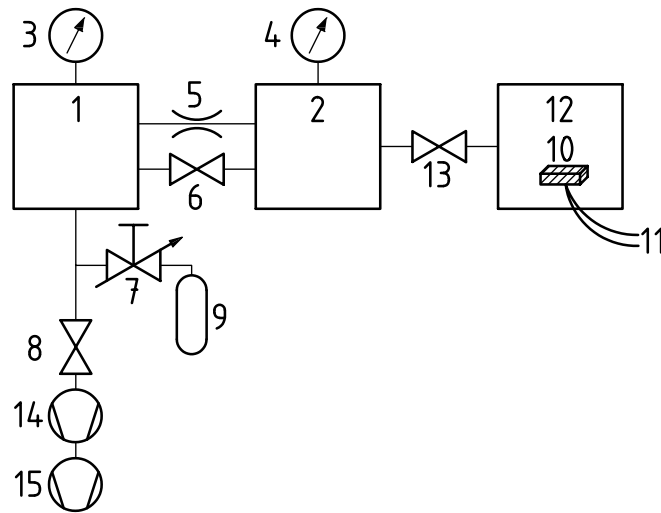
b) Method with sample chamber
