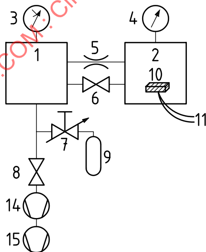
a) Method without sample chamber
