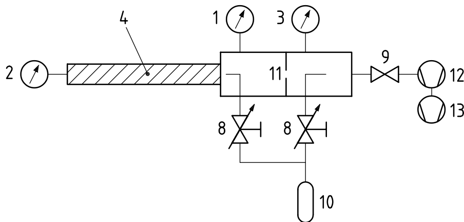
b) Method using orifice
