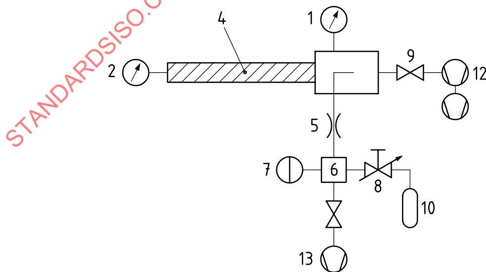
a) Method using leak element
