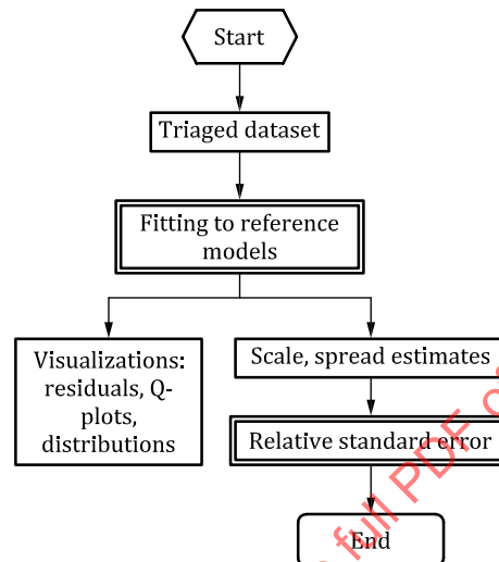
Figure 7 — Workflow for fitting particle size and shape distribution models to measured data
