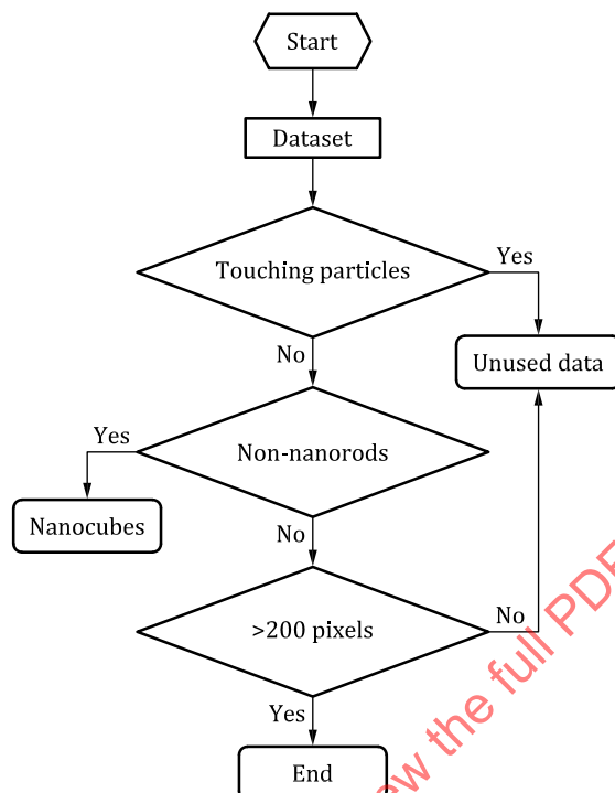
Figure 5 — Example of raw data triage for gold nanorod sample (see Annex D )
