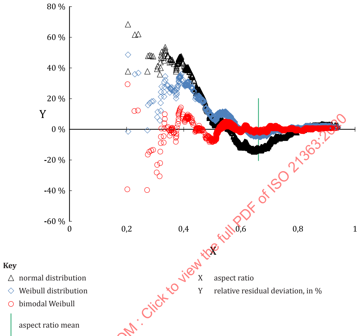
Figure F.3 — Normal, Weibull and bimodal Weibull fits to an aspect ratio distribution (Lab 1)
