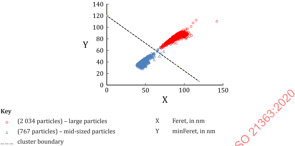
Figure C.5 — Size-size cluster analysis
