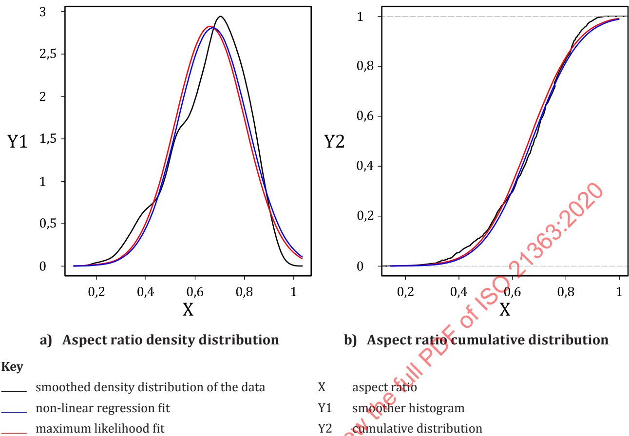
Figure F.2 — Density and cumulative distributions of aspect ratio (Lab 1)
