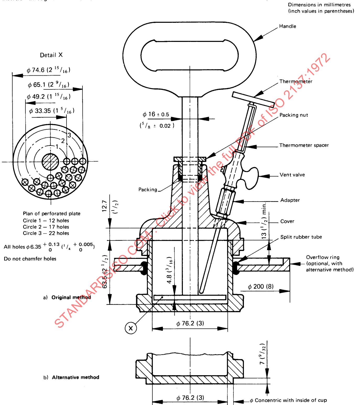
FIGURE 3 — Grease worker
