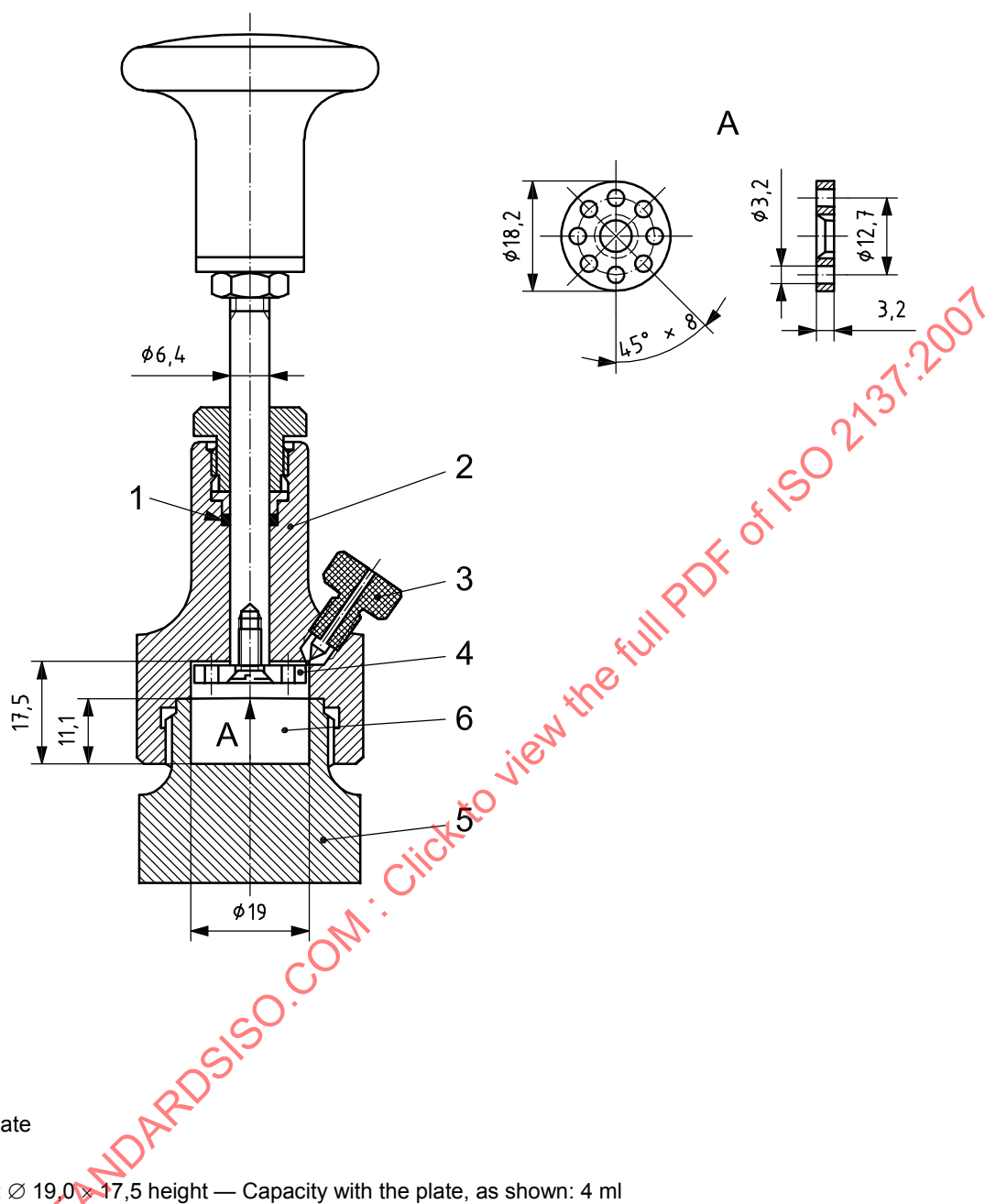
Figure 8 — One-quarter-scale grease worker
