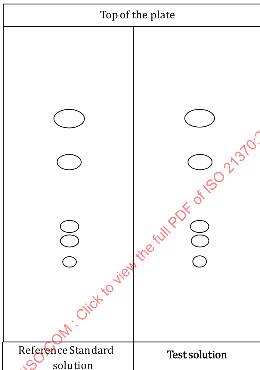
Figure A.1 — Schematic diagram of typical TLC chromatograms of Dendrobium officinale stem
