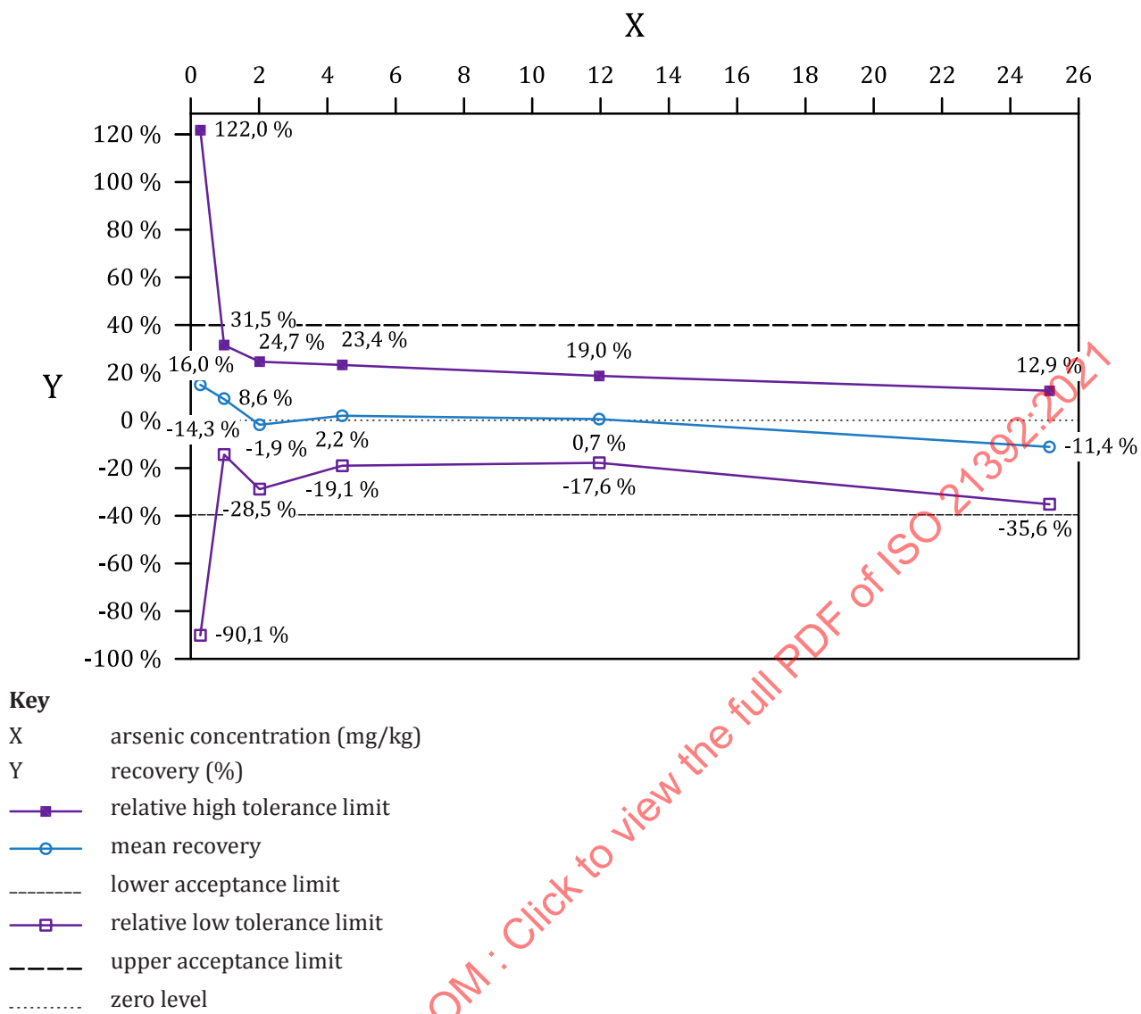
Figure A.4 — Accuracy profile for arsenic validating the method in the range 0,9 mg/kg to 25,1 mg/kg
