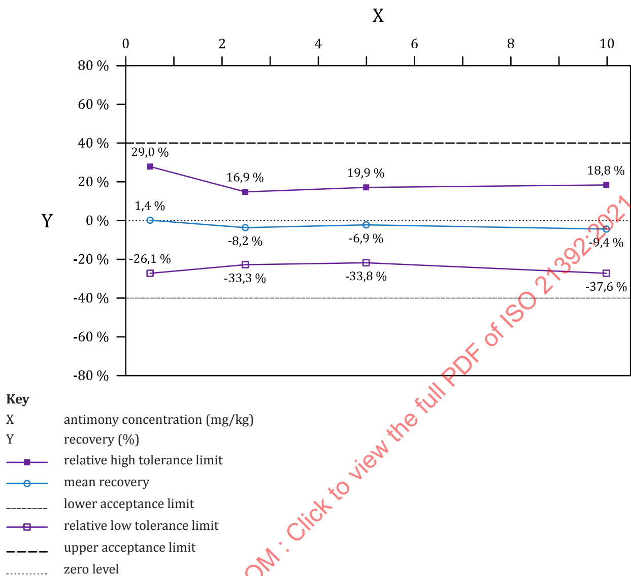
Figure A.6 — Accuracy profile for antimony validating the method in the range 0,5 mg/kg to 10 mg/kg
