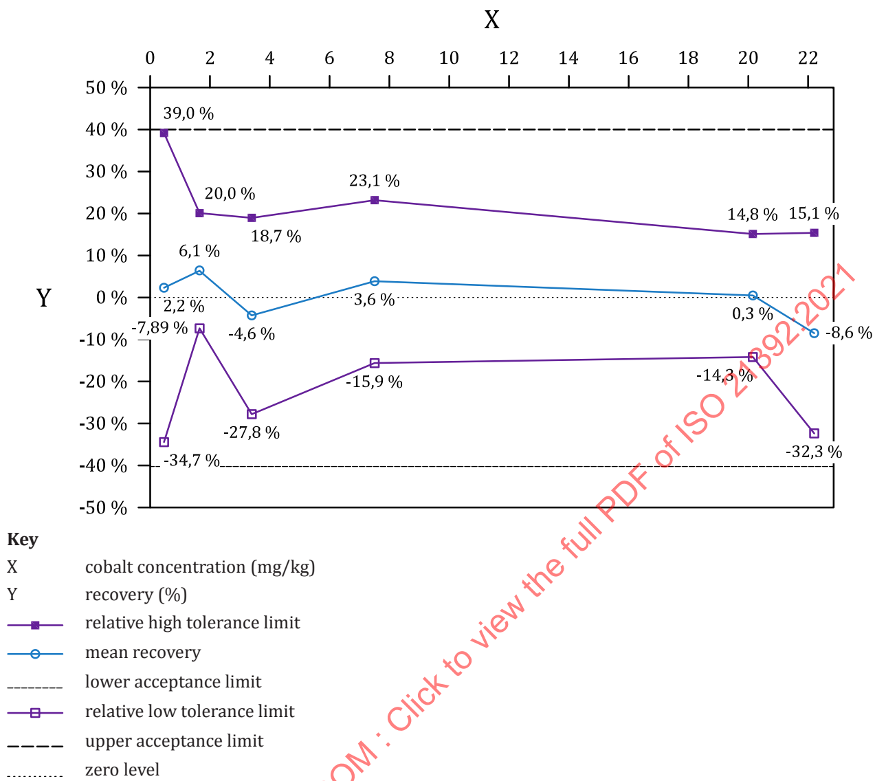
Figure A.2 — Accuracy profile for cobalt validating the method in the range 0,4 mg/kg to 22,3 mg/kg
