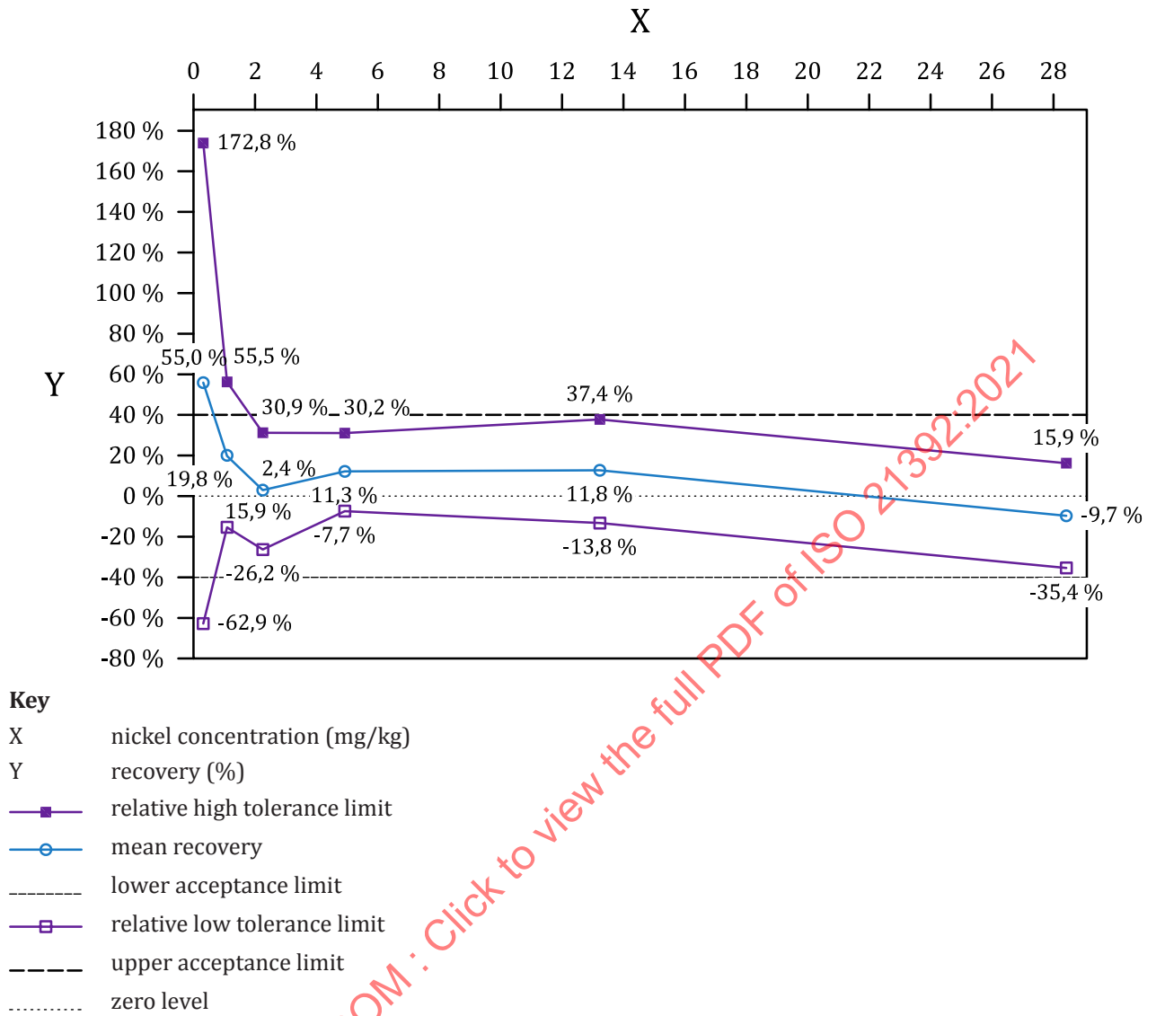
Figure A.3 — Accuracy profile for nickel validating the method in the range 1,8 mg/kg to 28,3 mg/kg
