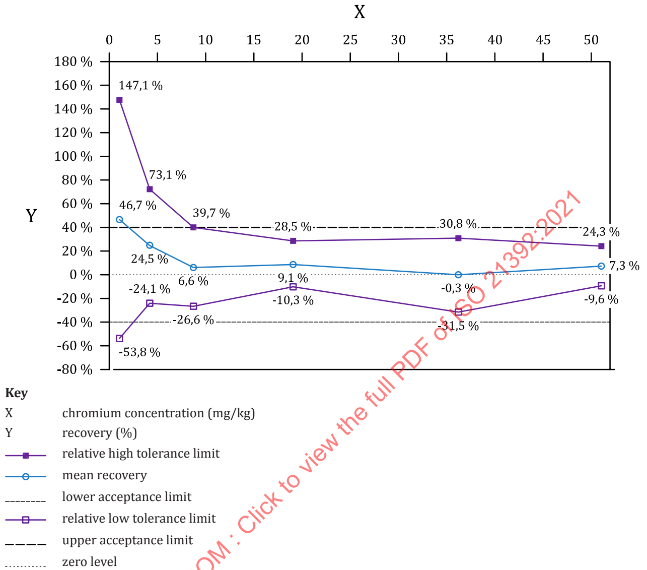
Figure A.1 — Accuracy profile for chromium validating the method in the range 8,6 mg/kg to 51 mg/kg
