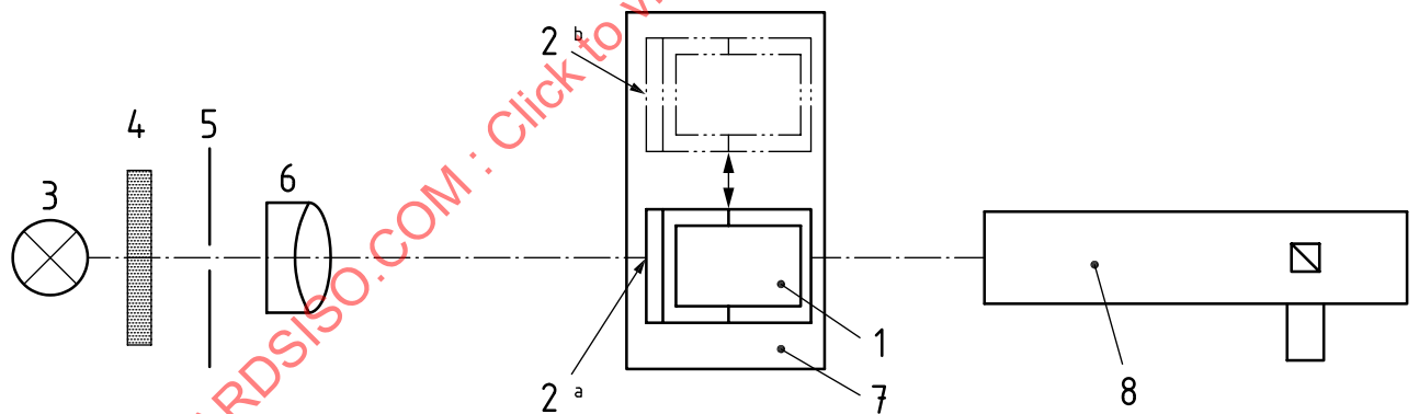
Figure C.3 — Outline of V-block alternative measurement equipment, side view
