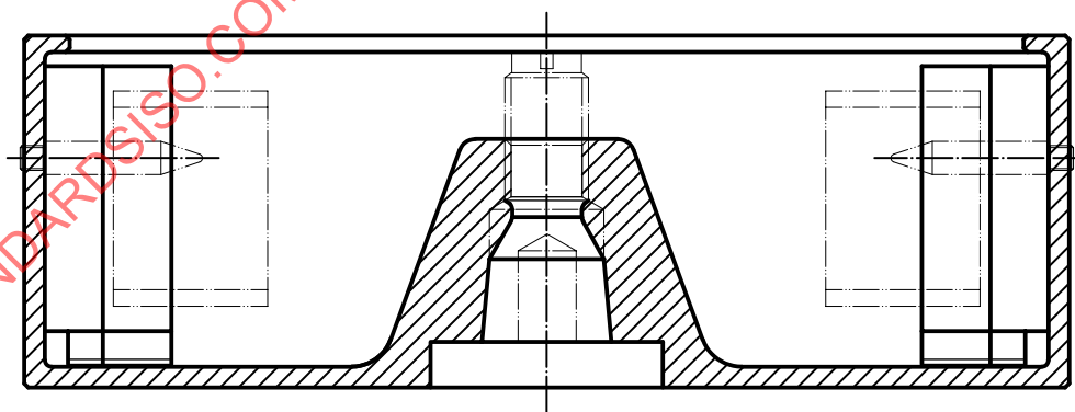
Figure A.3 — Centrifuge
