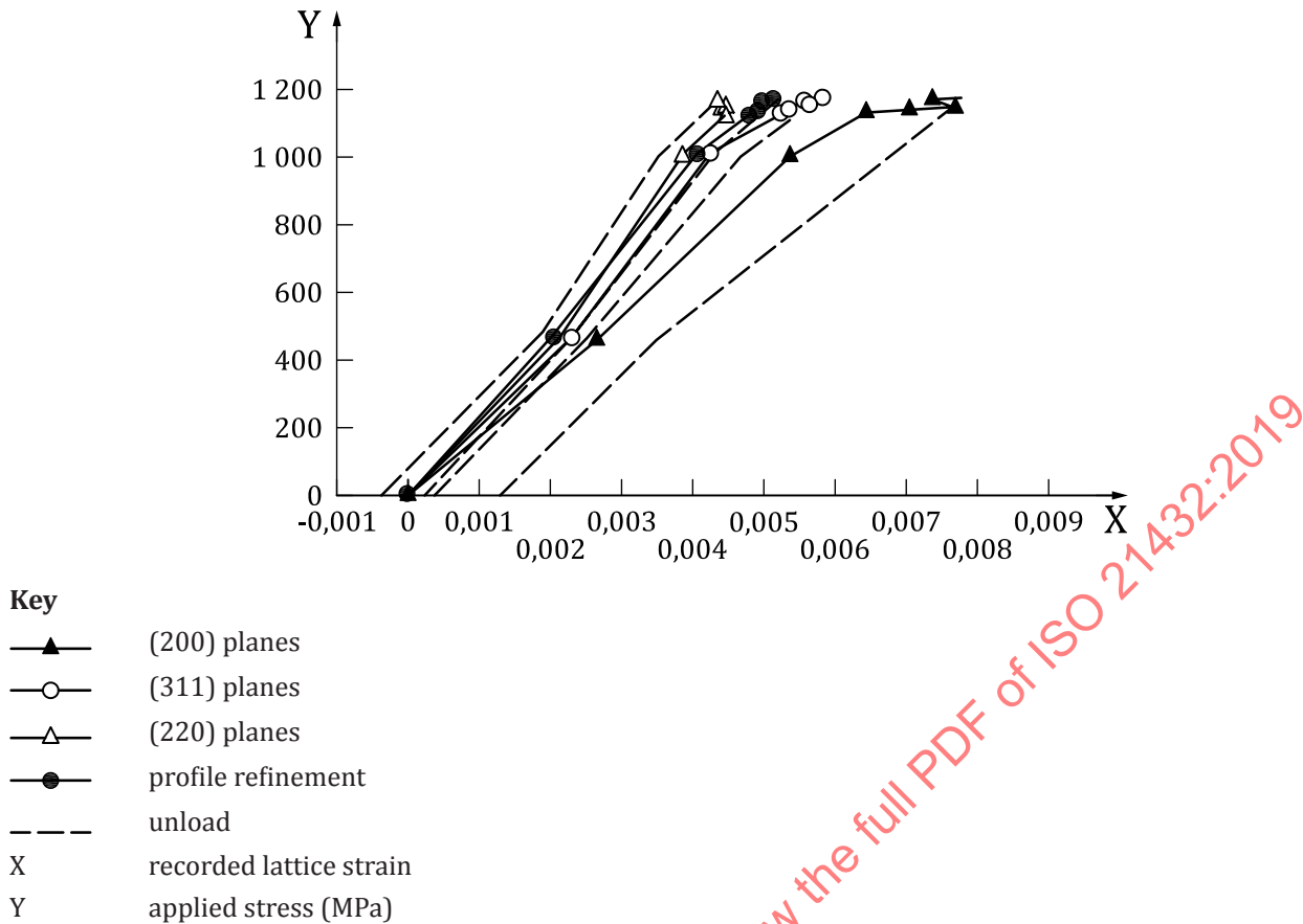
Figure 7 — Effect of yielding on the response of different crystallographic planes to the loading and unloading of a tensile bar of a nickel alloy [4]
