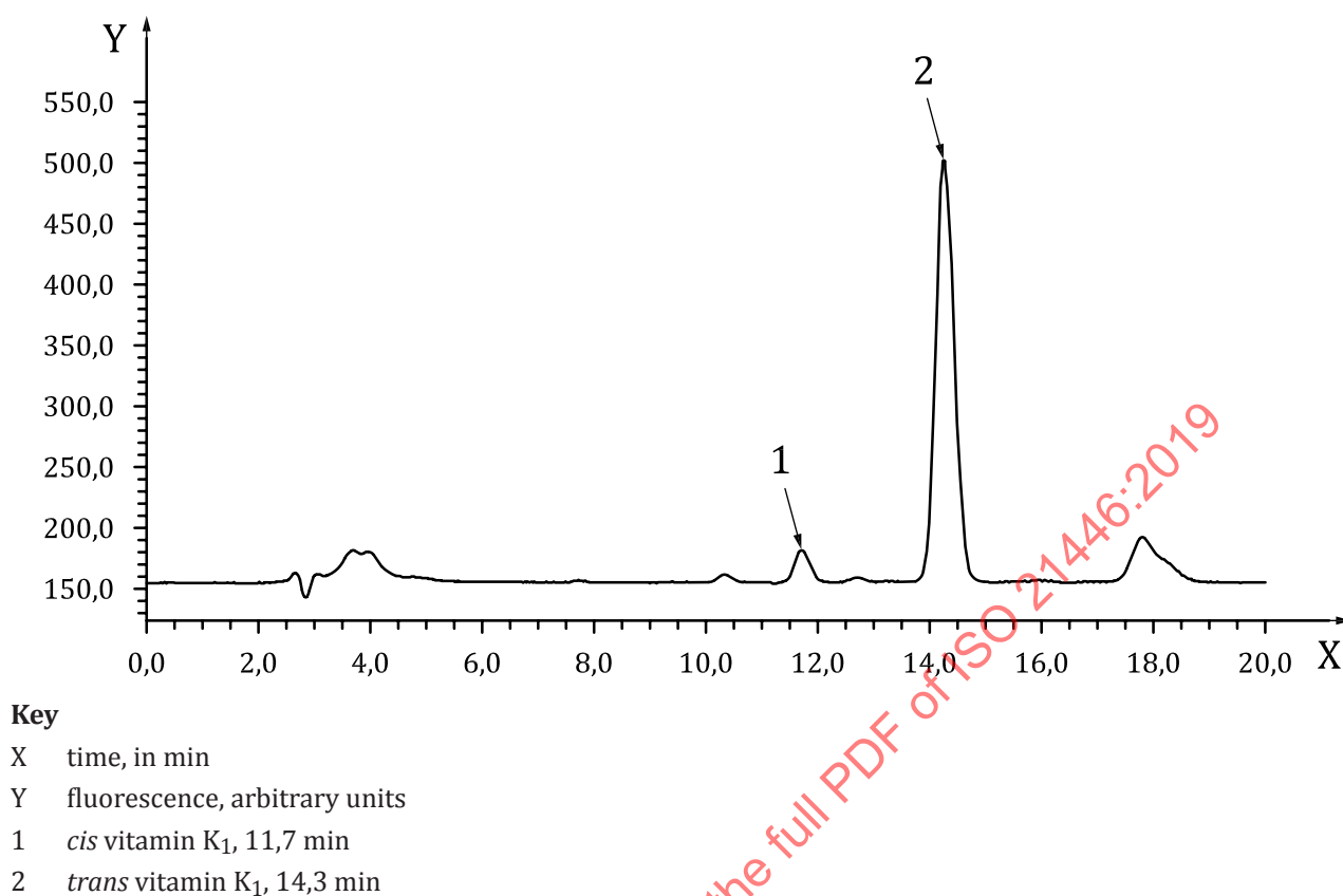
Figure A.2 — Chromatogram of SRM 1849a
