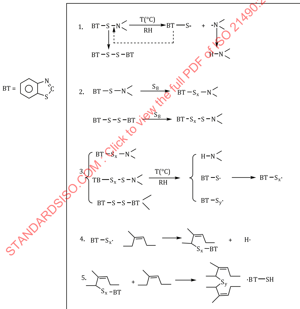
Figure A.1 — Reaction of sulfenamides during the curing of a rubber compound
