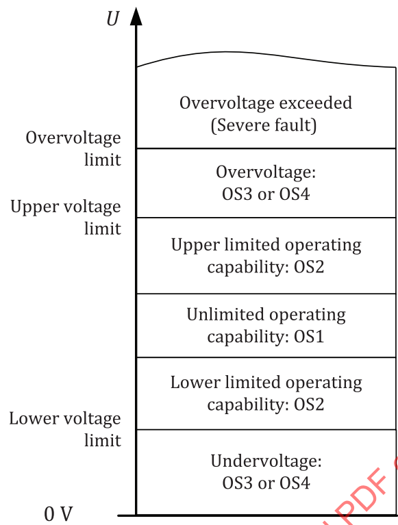
Figure 2 — Component operating status at a voltage sub-class
