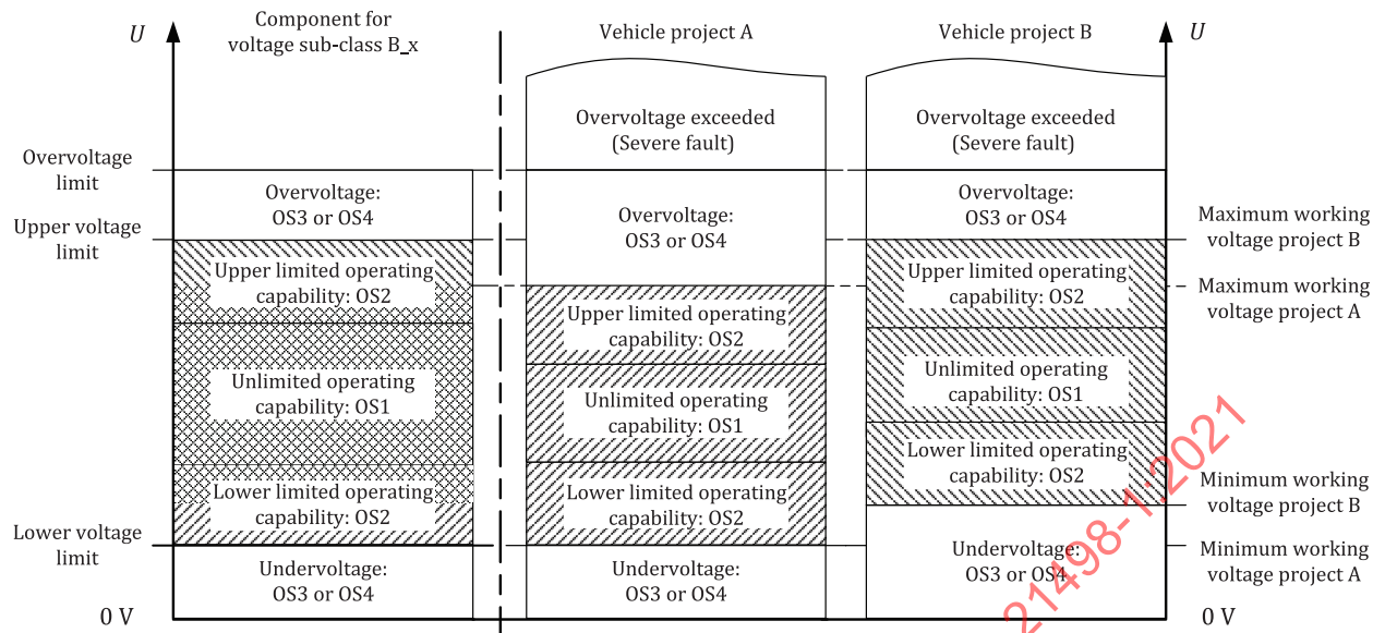
Figure 3 — Use of a component for voltage sub-class B x for different vehicle projects — Example
