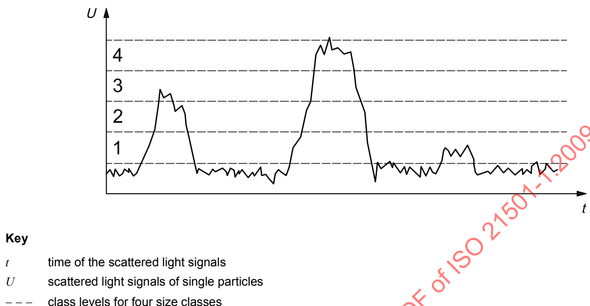
Figure A.4 — Example of the output signal of an LSAS [5]
