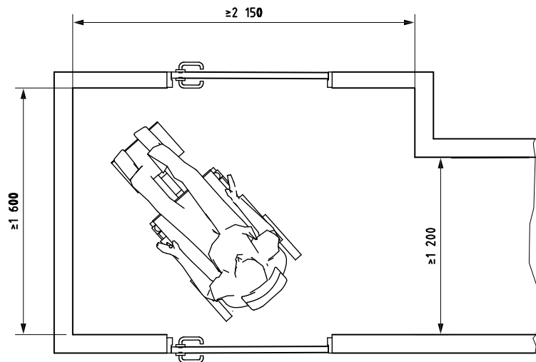
Figure 15 — Space required for a 180° turn in a corridor
