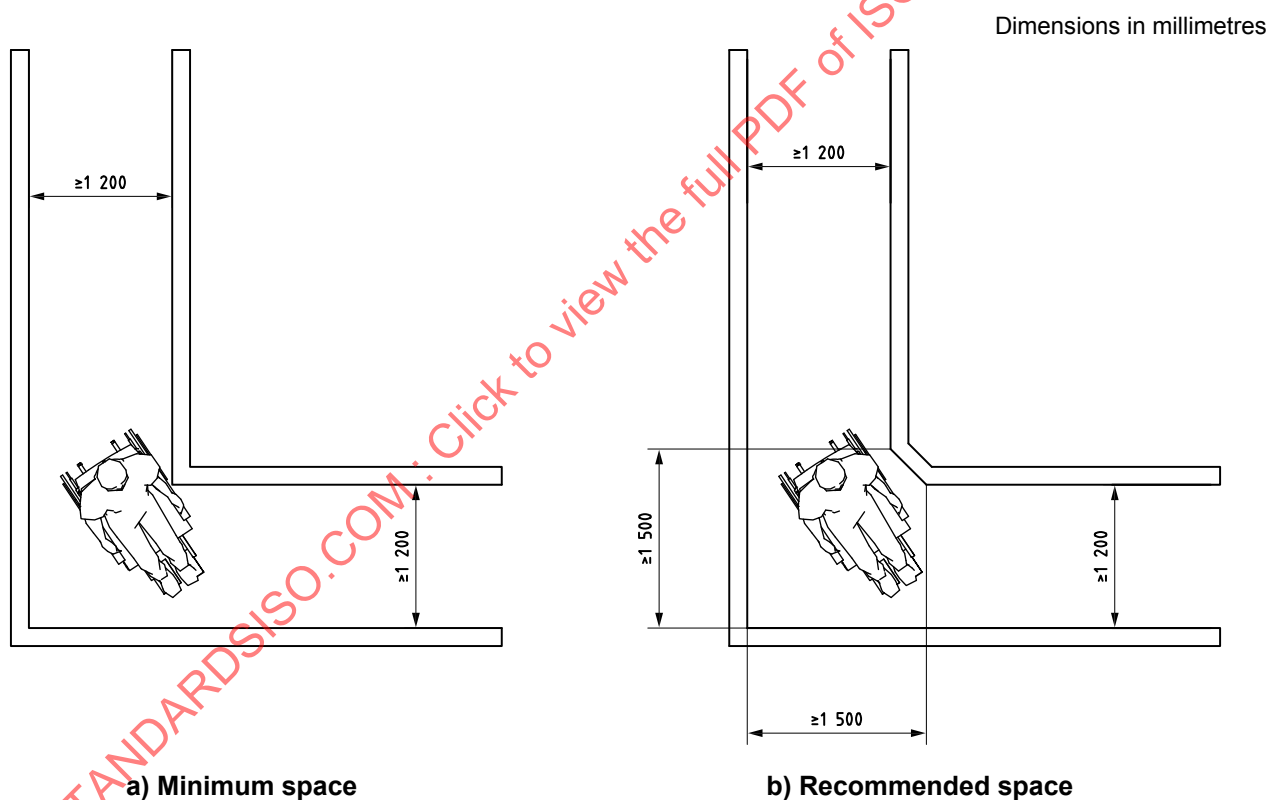
Figure 14 — Minimum and recommended space required for a 90° turn
