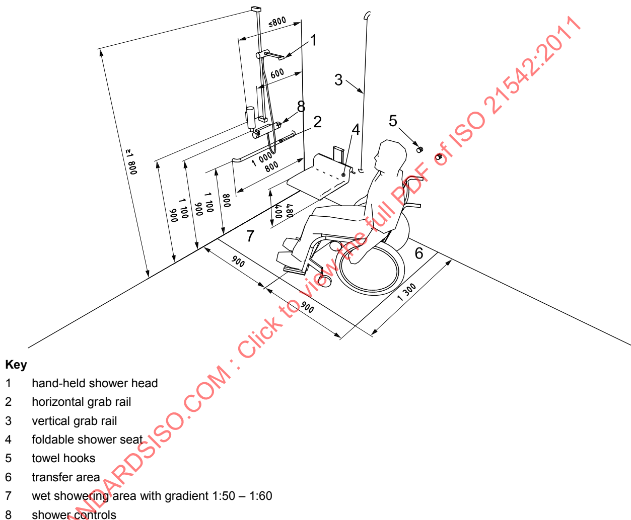
Figure 45 — Example of a shower place with grab rails, adjustable shower head and folding seat
