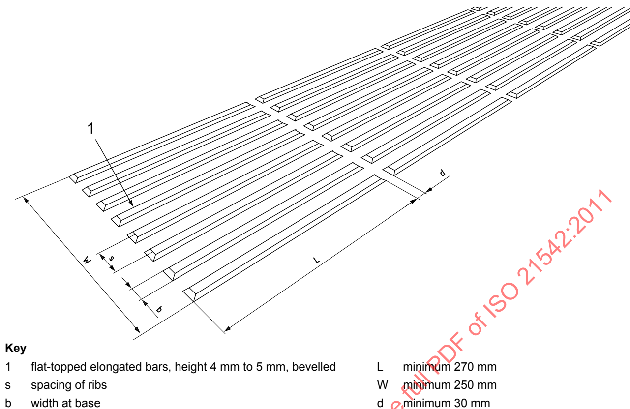
Figure A.3 — Spacing and dimensions of flat-topped elongated bars
