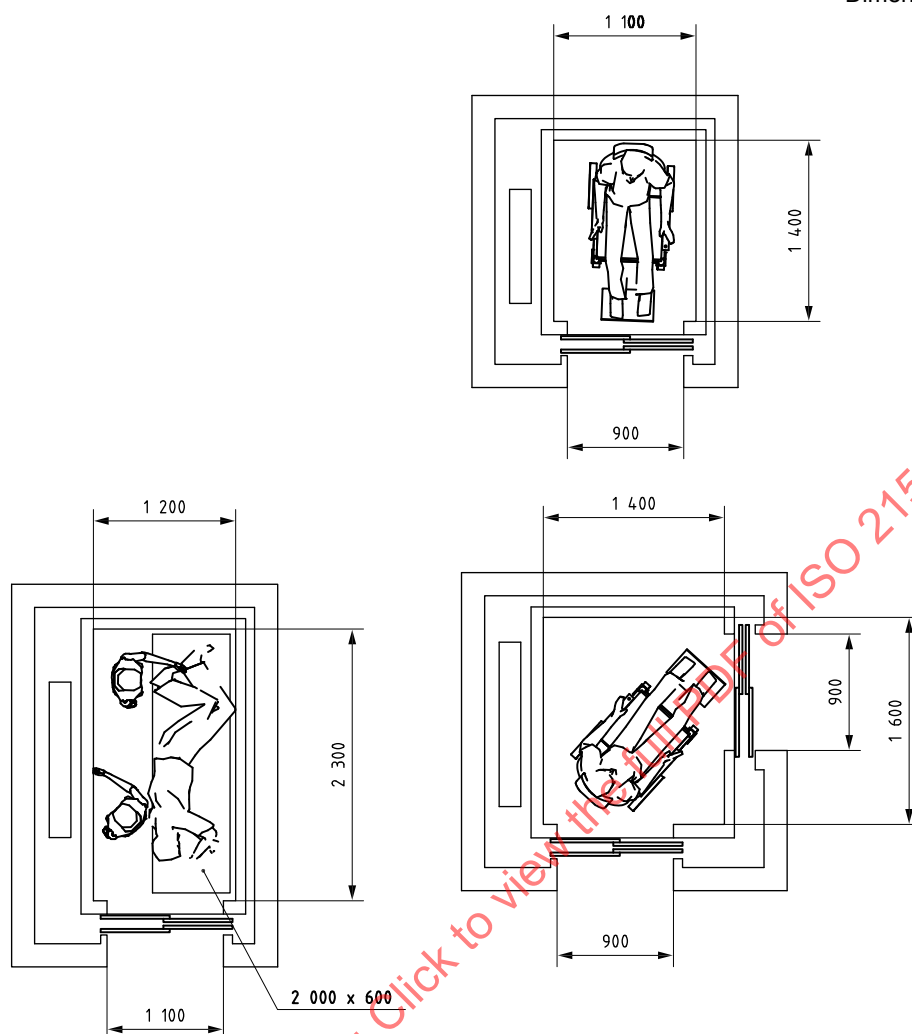
Figure 21 — Examples of lifts accommodating one person in a wheelchair, a person on a stretcher and a person performing a 90° turn between two adjacent lift doors
