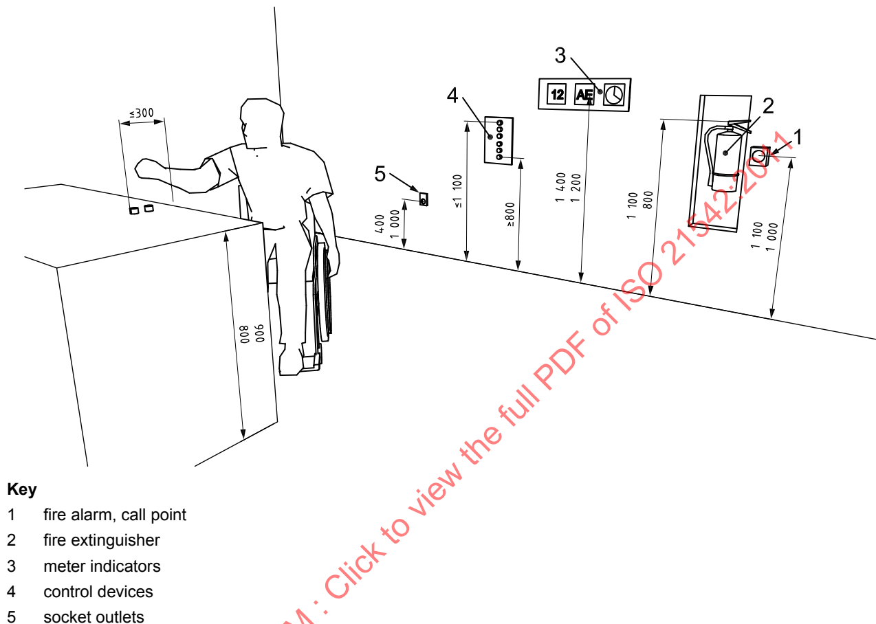
Figure 53 — Heights of switches, socket outlets, reading controls and controls on a horizontal surface
