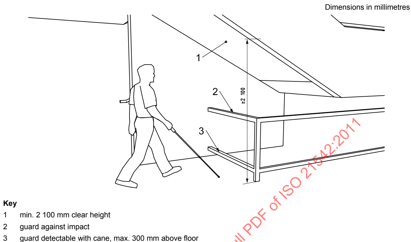
Figure 18 — Clear height under stairs
