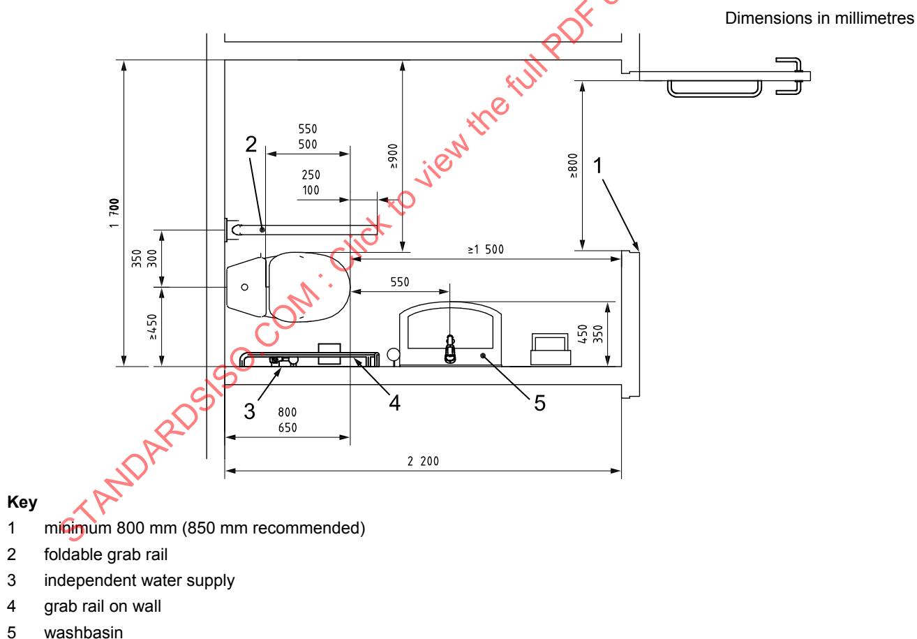
Figure 40 — Example of type C small corner toilet room
