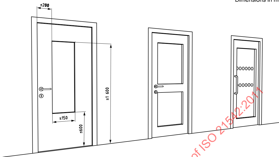
Figure 28 — Examples of doors with glazed viewing panels
