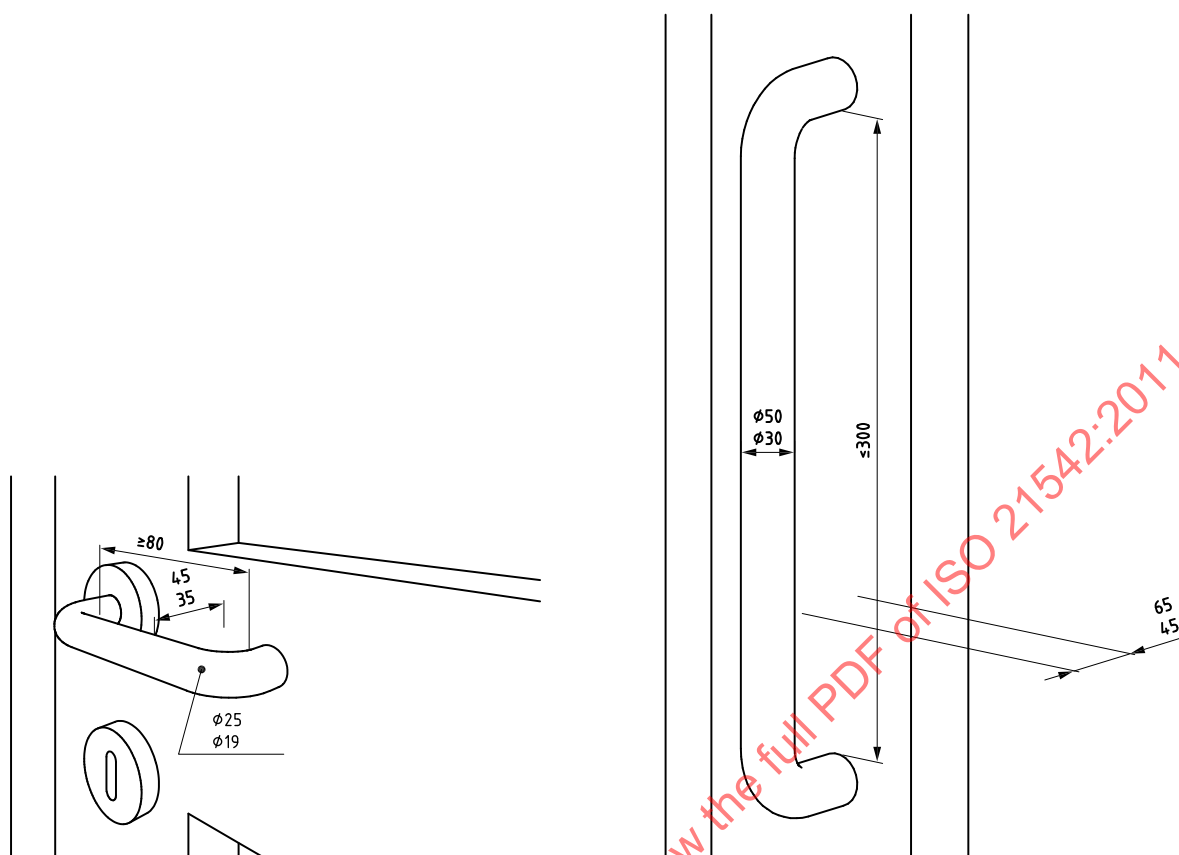
Figure 57 — Examples of D-lever and vertical door handles
