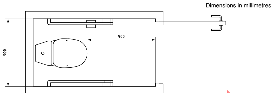
Figure 35 — Ambulant toilet
