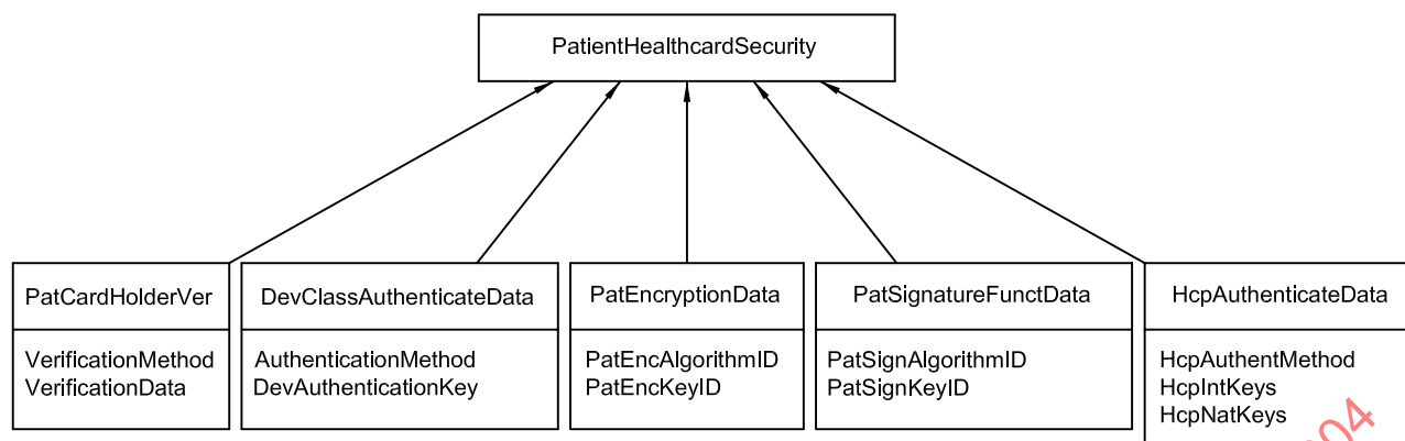
Figure 6 — The structure of “PatientHealthcardSecurity”
