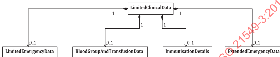
Figure 2 — Structure of LimitedClinicalData
