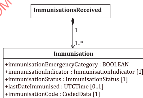
Figure 5 — Structure of ImmunisationsReceived
