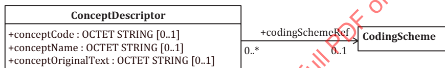
Figure 10 — Structure of ConceptDescriptor
