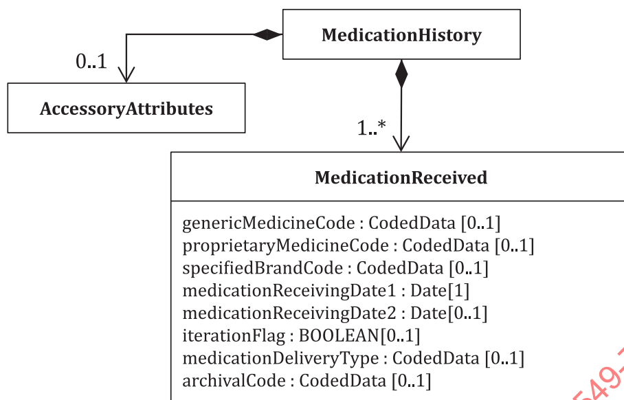
Figure 4 — Structure of MedicationHistory
