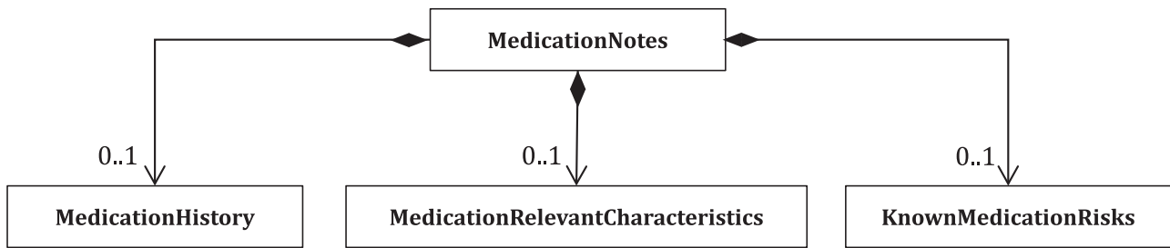
Figure 3 — Structure of MedicationNotes
