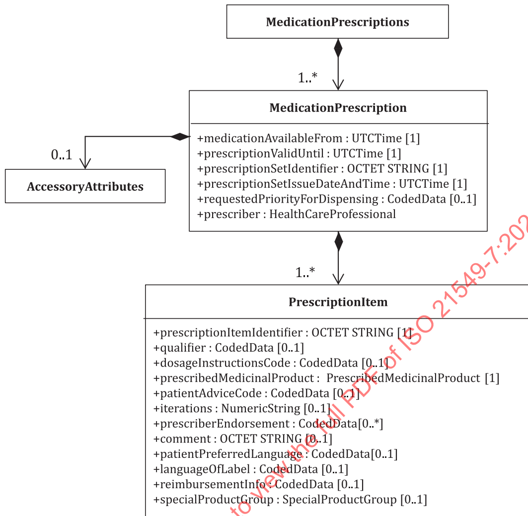
Figure 7 — Structure of MedicationPrescription
