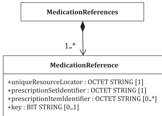
Figure 24 — Structure of MedicationReferences
