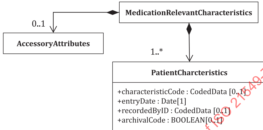
Figure 5 — Structure of MedicationRelevantCharacteristics
