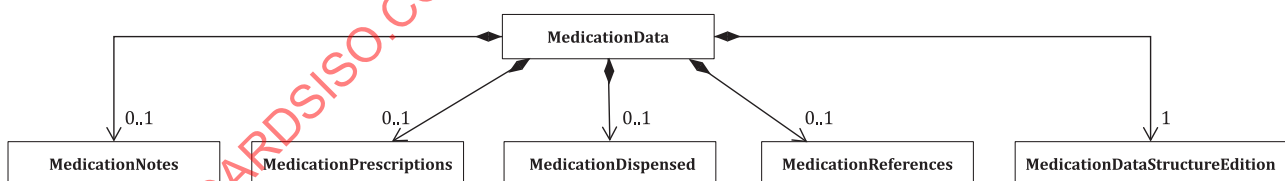
Figure 2 — Structure of MedicationData
