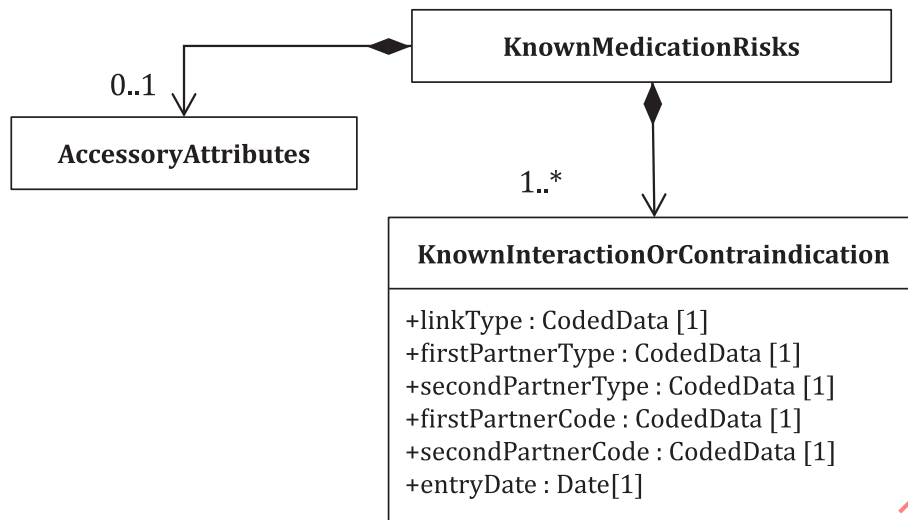
Figure 6 — Structure of KnownMedicationRisks
