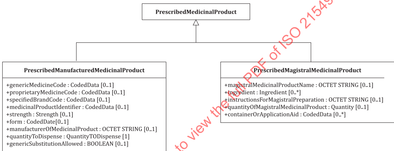
Figure 8 — Structure of PrescribedMedicinalProduct
