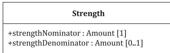
Figure 10 — Structure of Strength
