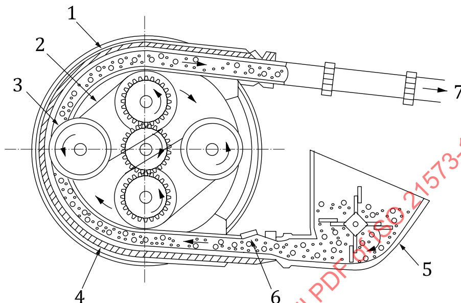
Figure A.5 — Structure and principle of operation of the Skirt-valve system
