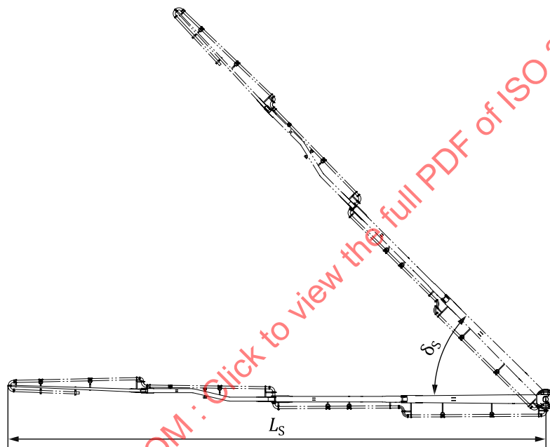
Figure 14 — Slewing motion of concrete-placing boom
