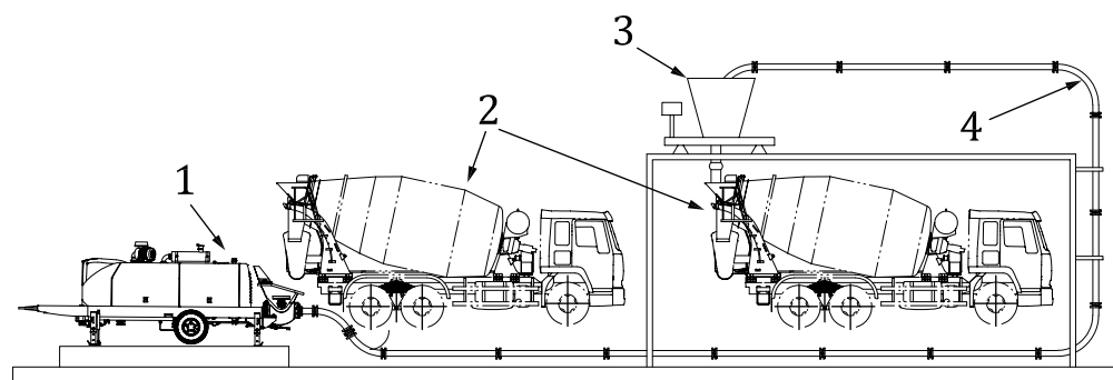
a) Concrete pump without concrete-placing boom
