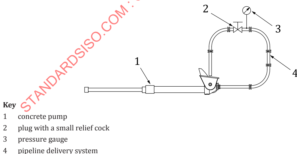
Figure 7 — Delivery pressure measuring system
