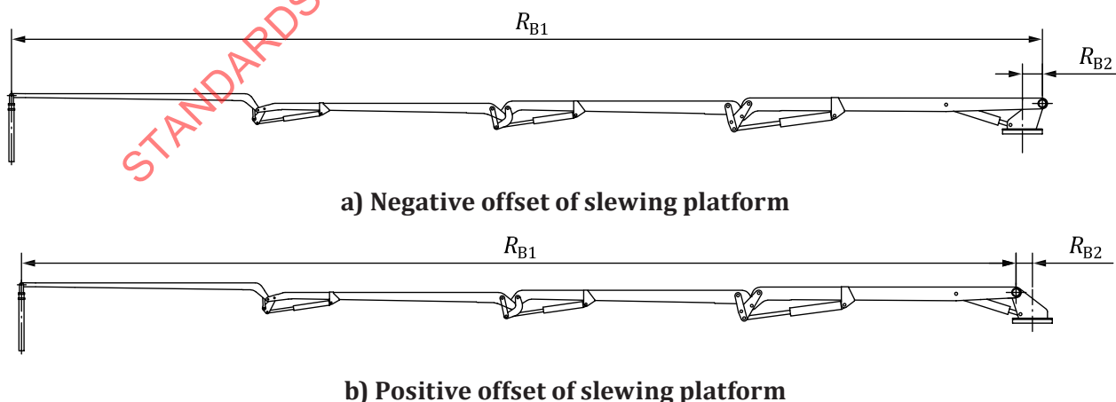
Figure 9 — Placing radius
