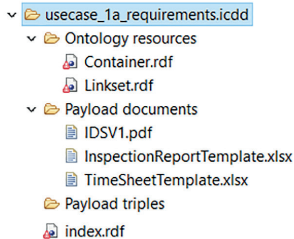
Figure A.2 — Example of a container structure
