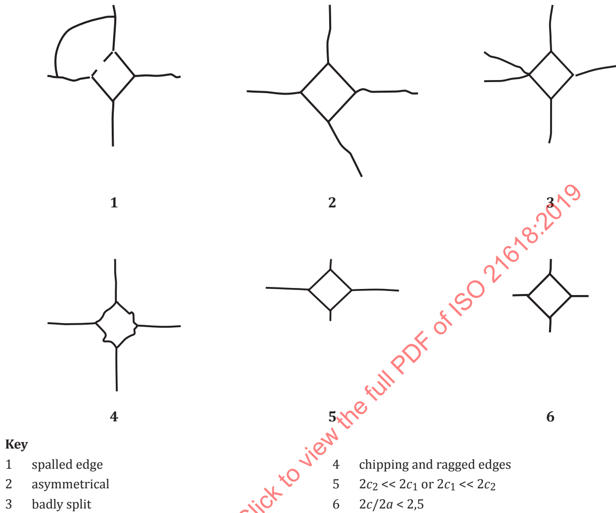
Figure 2 — Guidelines for the unacceptable indentations
