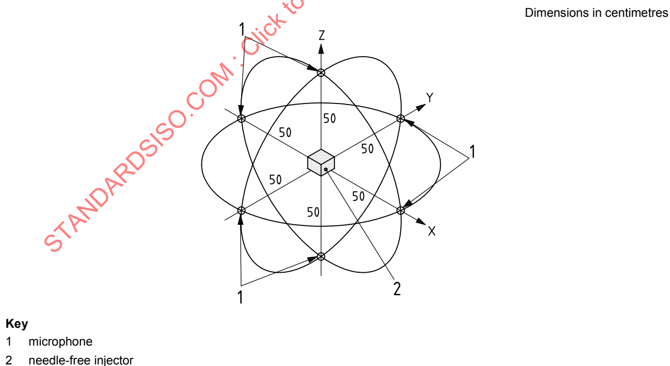
Figure 1 — Microphone positions
