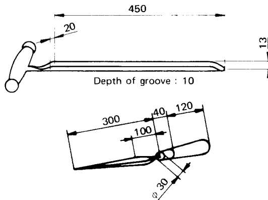
FIGURE 1 — Sampling spears (open triers)
