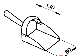
Figure 2 — Hand-scoop
