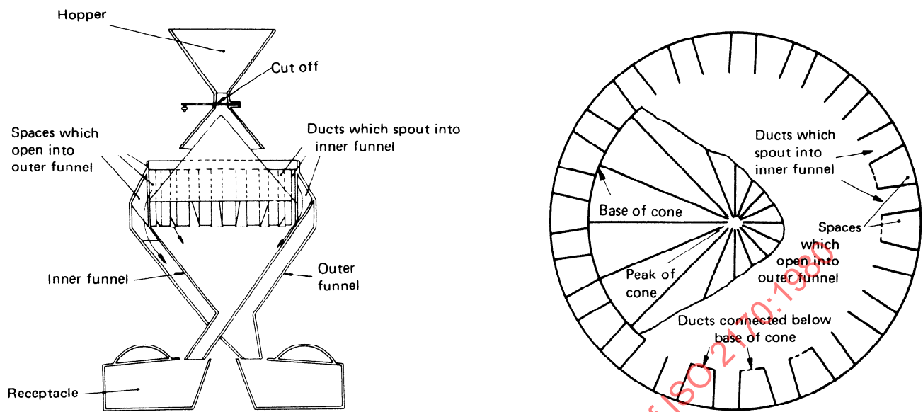
Figure 8 — Conical divider
