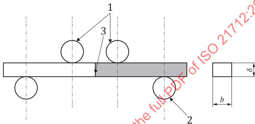
a) Type A specimen
