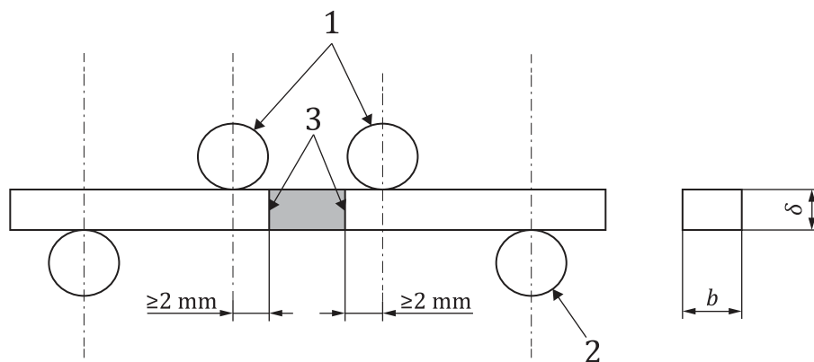
c) Type B specimen (two interfaces are examined simultaneously)
