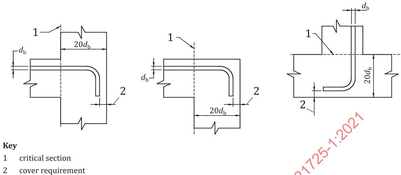
Figure 30 — Minimum standard hook anchorage distance
