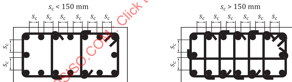
Figure 35 — Arrangement of ties in a tied column section
