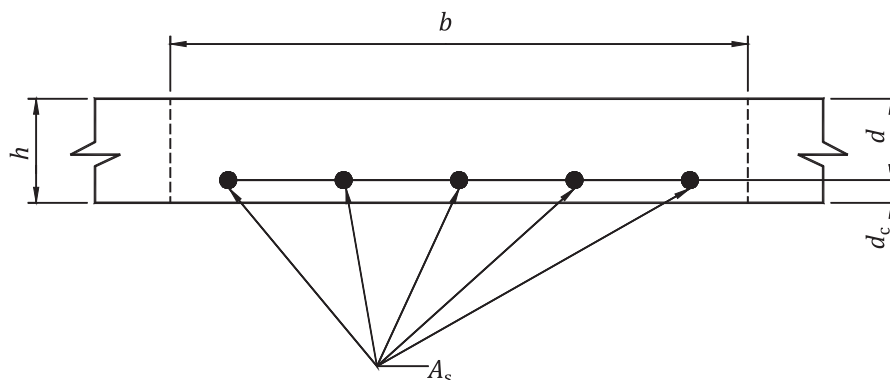
Figure 31 — Slab or footing section
