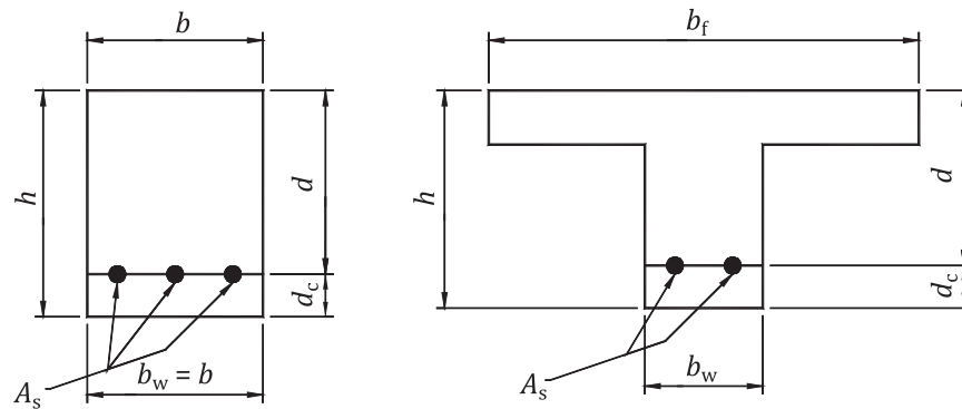
Figure 32 — Rectangular section and T-shaped section with flange in compression
