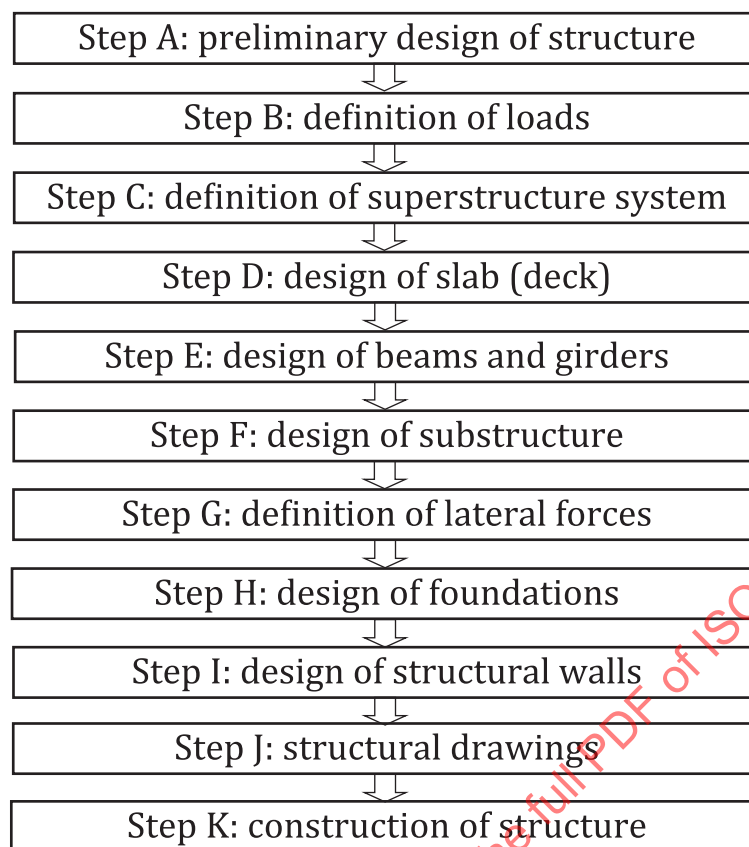
Figure 1 — Design and construction procedure
