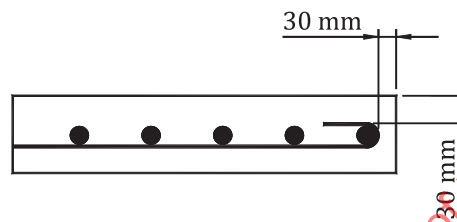
Figure 13 — All types of reinforcement of solid slabs, structural concrete walls or joists, when not exposed to weather or in contact with ground (Minimum concrete cover: 30 mm)
