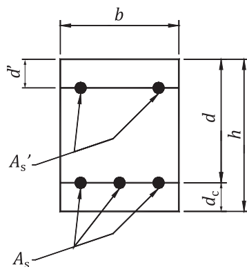
Figure 34 — Section with tension and compression reinforcement
