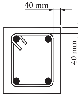
Figure 12 — All types of reinforcement of girders, beams, or columns, when not exposed to weather or in contact with ground (Minimum concrete cover: 40 mm)
