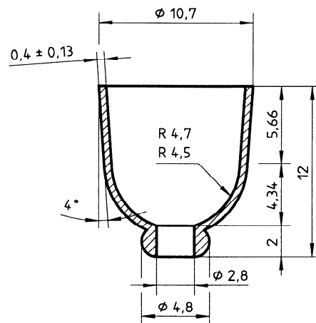
Figure 1 — Grease cup
