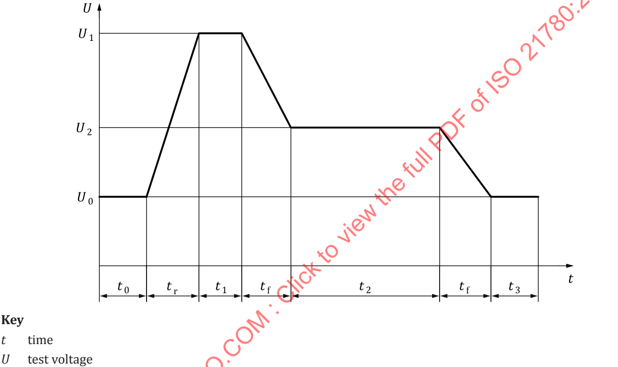
Figure 5 — Test profile for test-03: short term overvoltage
