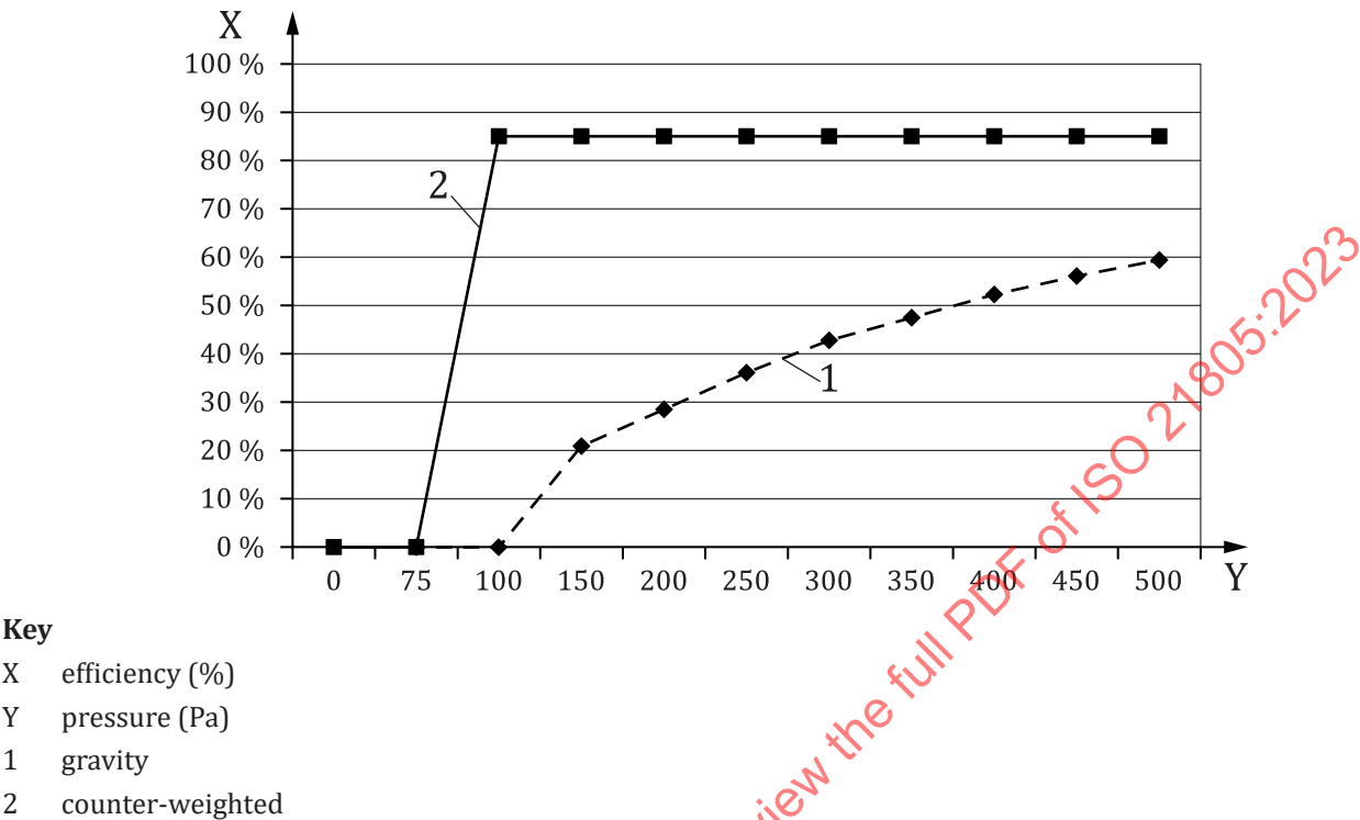
Figure 5 — Efficiency of pressure-relief vents
