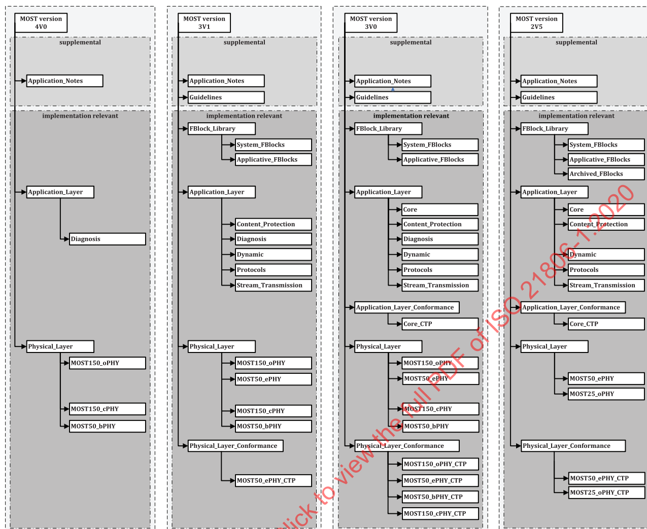
Figure 4 — MOST versions directory structure
