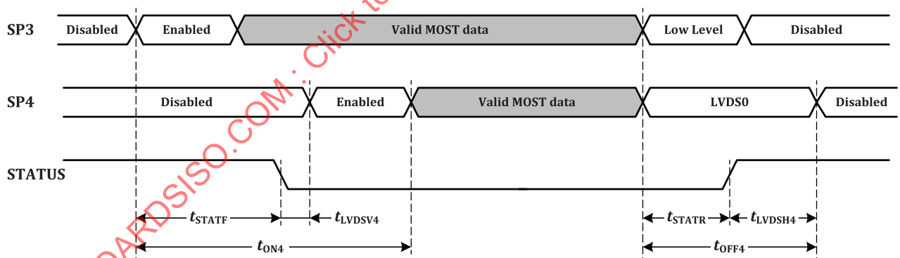
Figure 24 — CEC timing diagram
