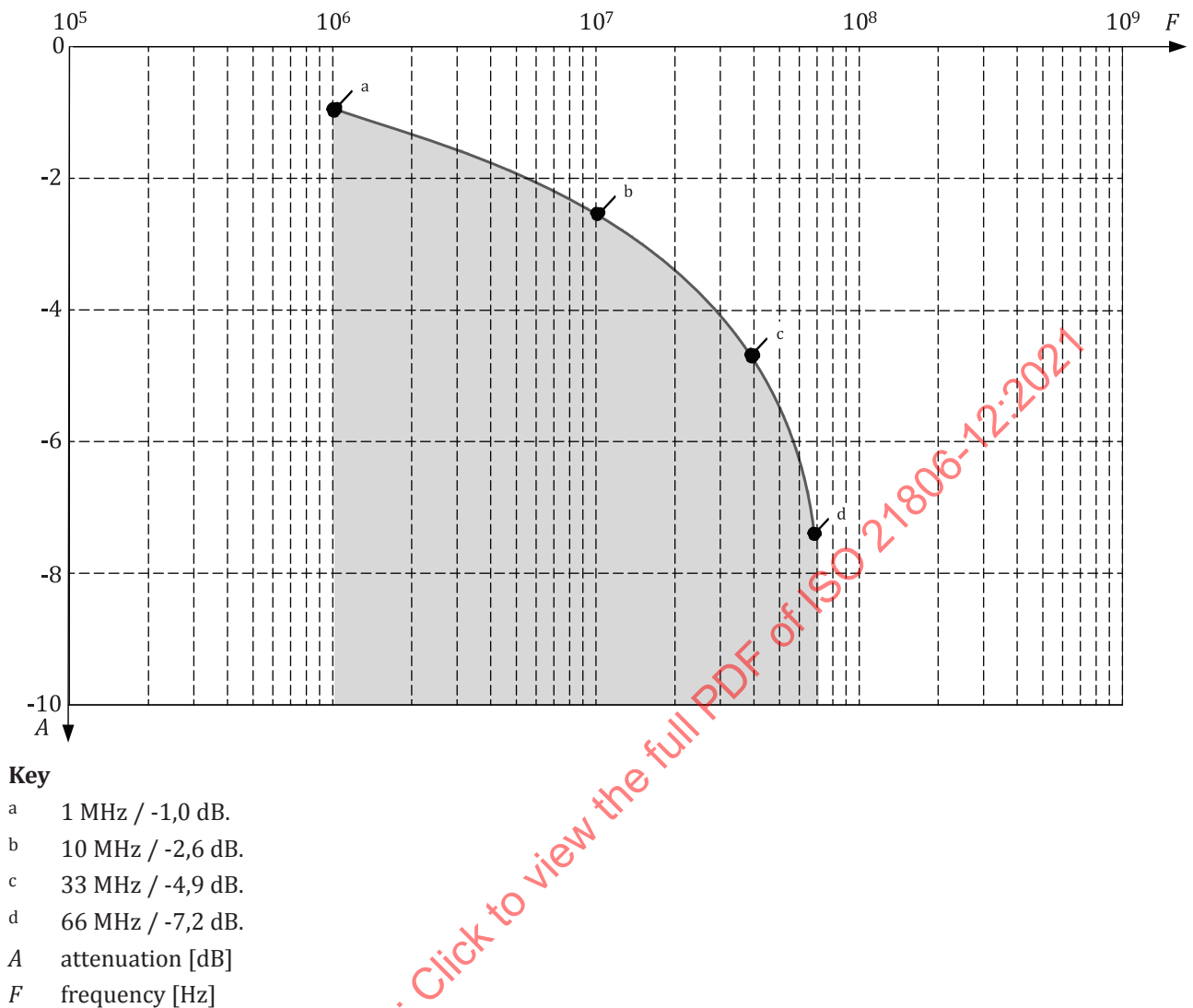
Figure 17 — Attenuation limit
