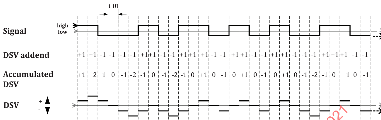
Figure 10 — DSV calculation
