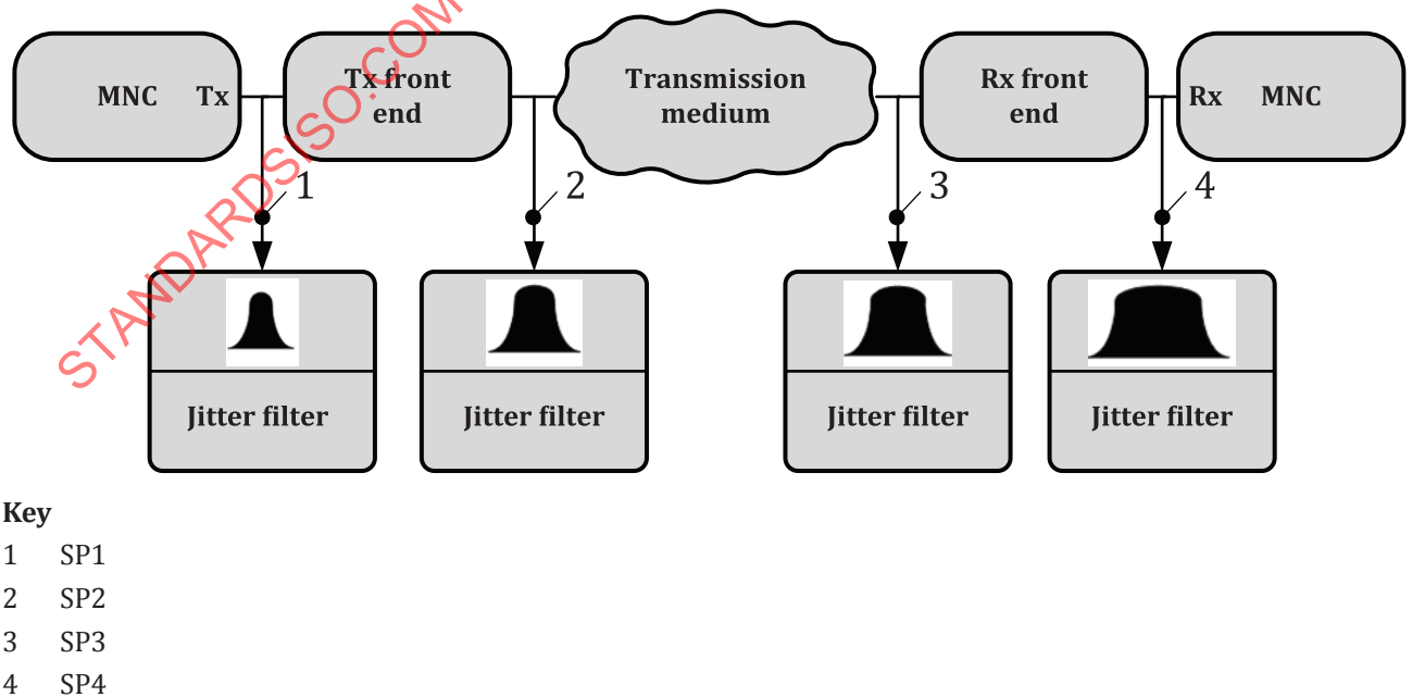
Figure 7 — Illustration of transferred jitter accumulation at various SPs in a link
