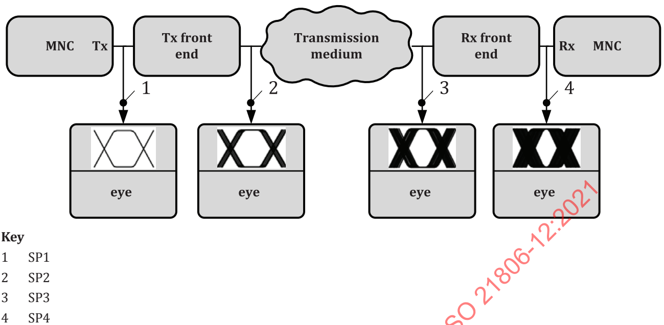
Figure 6 — Illustration of eye diagrams at SPs in a link
