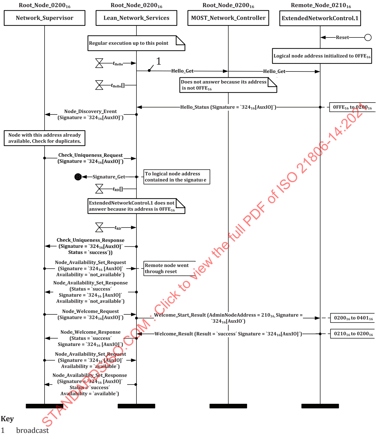
Figure 8 — Reset detection example MSC
