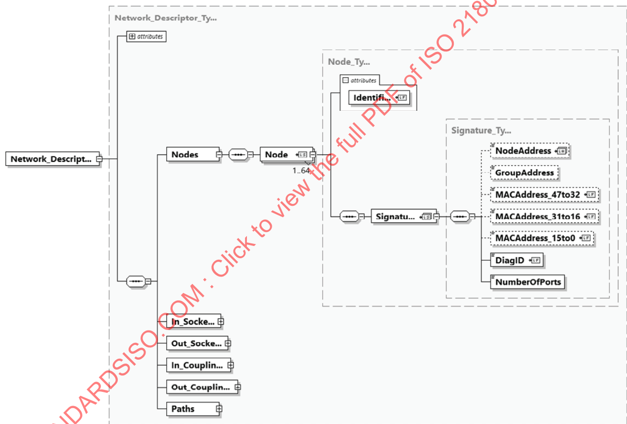
Figure B.1 — Network descriptor XML schema — Nodes
