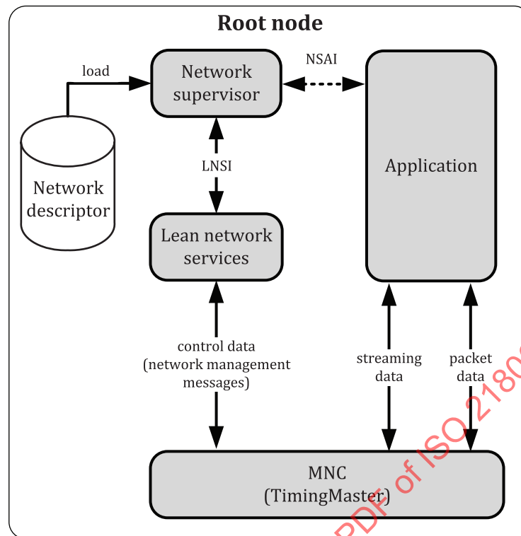
Figure 4 — Root node
