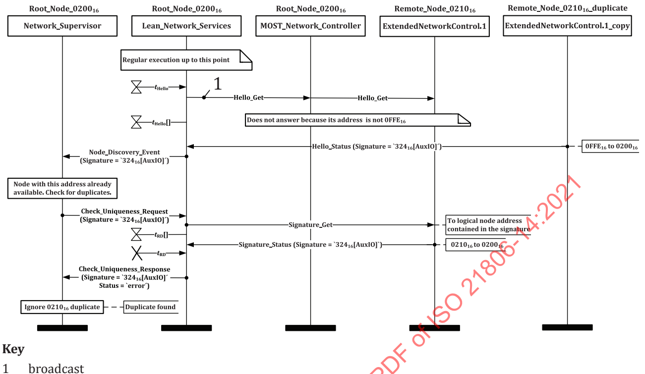
Figure 9 — Duplicate address detection example MSC
