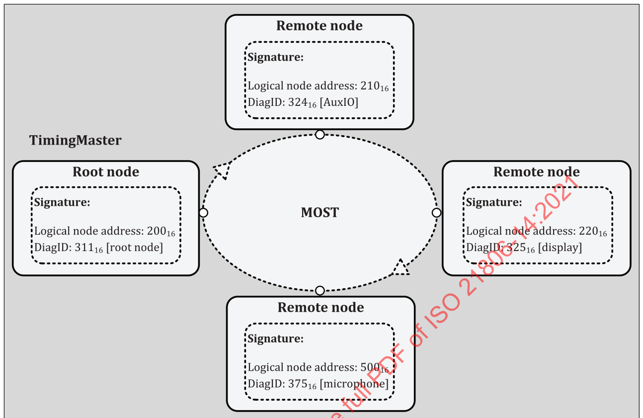
Figure 6 — Node discovery example configuration
