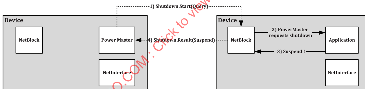
Figure 19 — Prevention of switching off MOST network via Shutdown.Result(Suspend)
