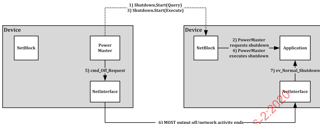
Figure 20 — Switching off MOST network by starting the Shutdown method in every NetBlock FBlock
