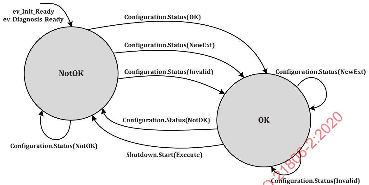
Figure 18 — NetworkSlave determines the central registry state in s_NetInterface_Normal_Operation
