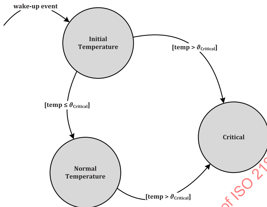
Figure 25 — Mandatory over-temperature behaviour
