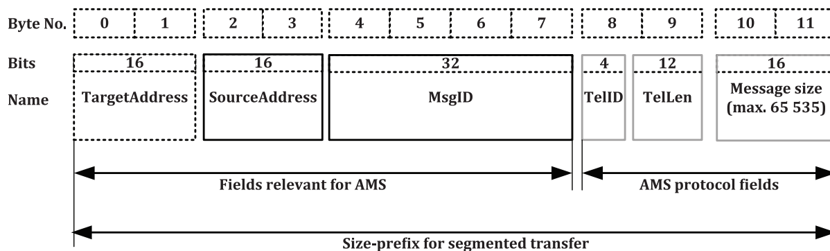
Figure 5 — Size-prefix for segmented transfer
