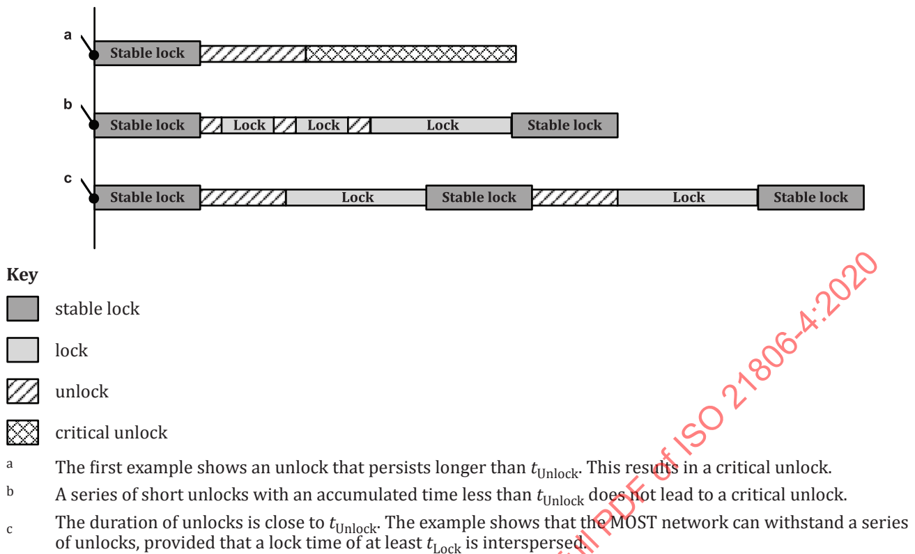
Figure 14 — Examples of the behaviour when unlocks occur
