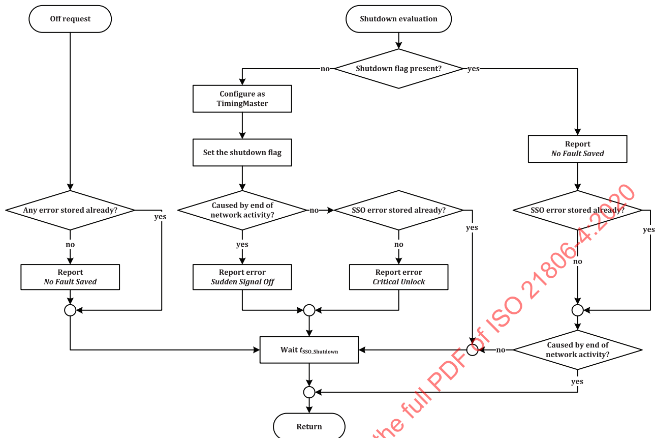
Figure 15 — Procedure “Off request” and procedure “Shutdown evaluation”
