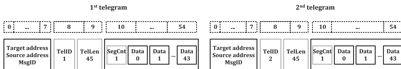
Figure 7 — Segmented transfer example with entire available payload used
