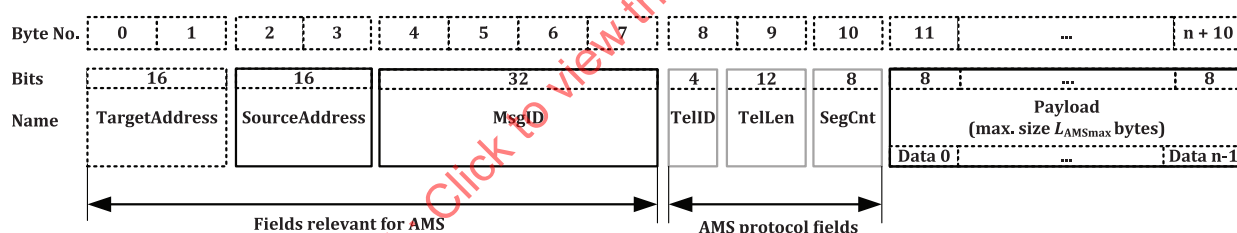
Figure 6 — One telegram (n bytes payload) of a segmented transfer
