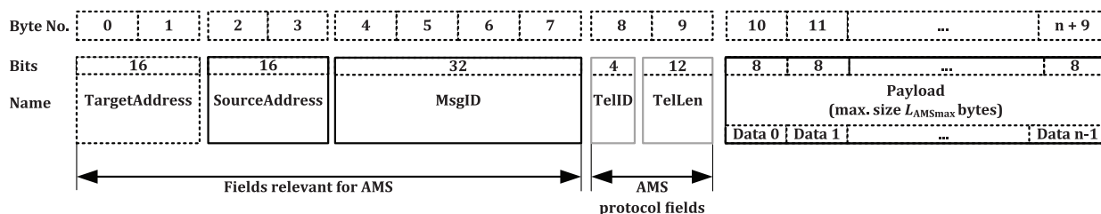
Figure 4 — Single transfer (n bytes payload)
