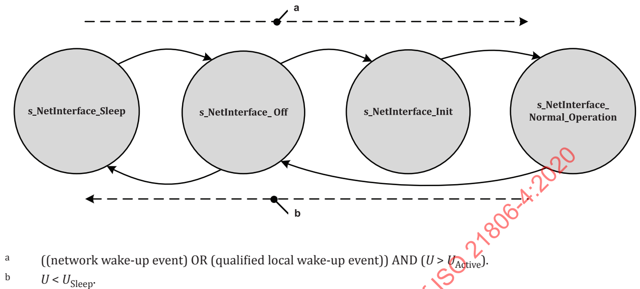
Figure 16 — Behaviour of a node depending on supply voltage
