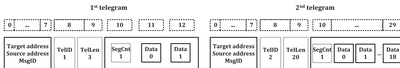
Figure 8 — Segmented transfer example with available payload not entirely used
