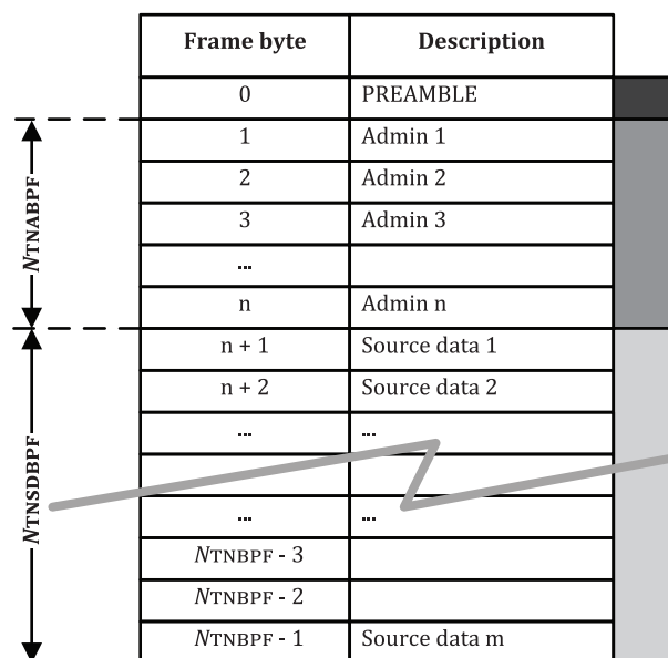
Figure 5 — Network frame — Structure
