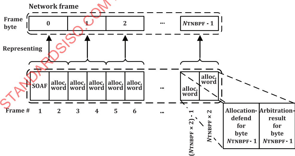
Figure 7 — Allocation words representing bytes of network frame
