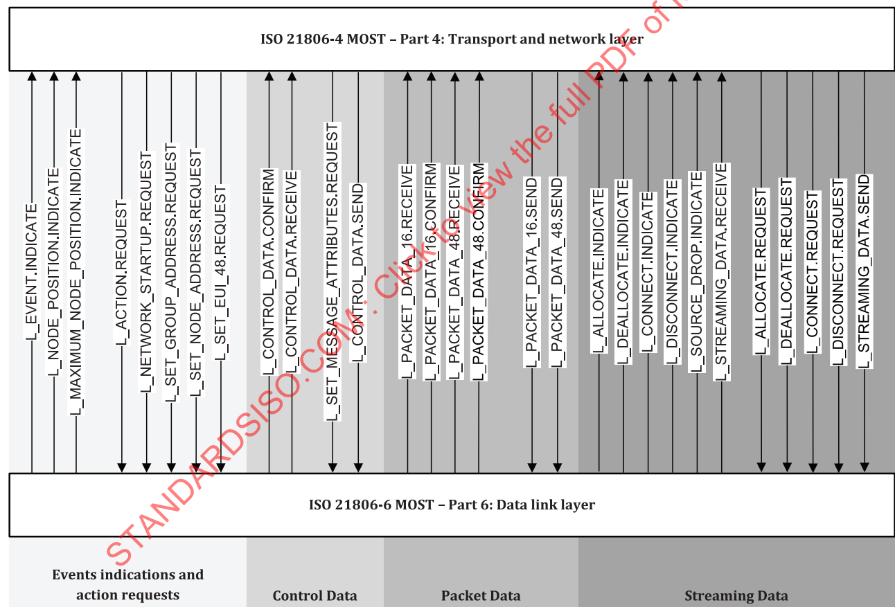
Figure 3 — Service interface to upper layers
