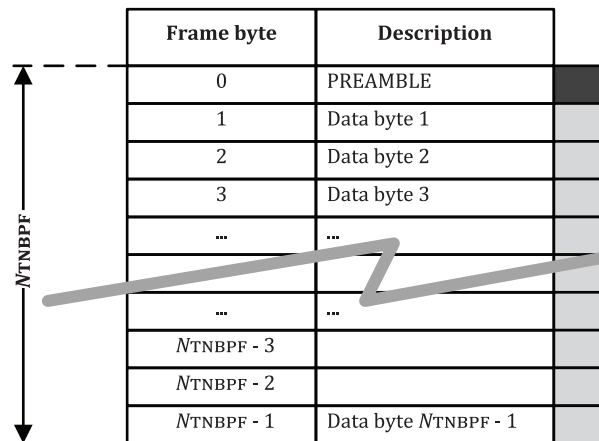
Figure 4 — Network frame
