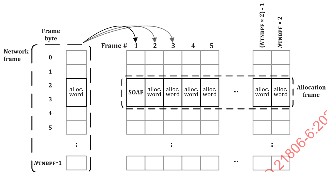
Figure 6 — Allocation words of subsequent network frames forming the allocation frame
