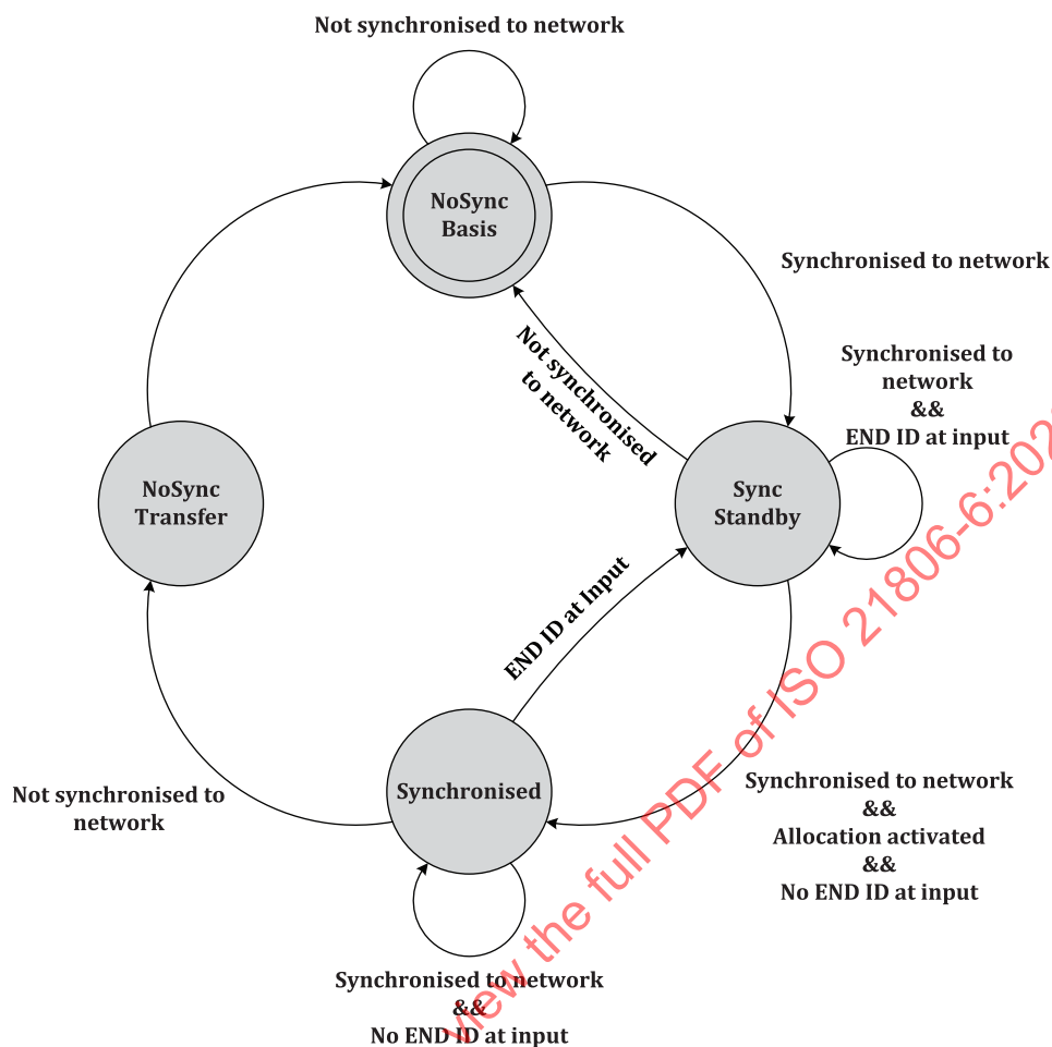
Figure 10 — Error handling of TimingMaster and TimingSlaves
