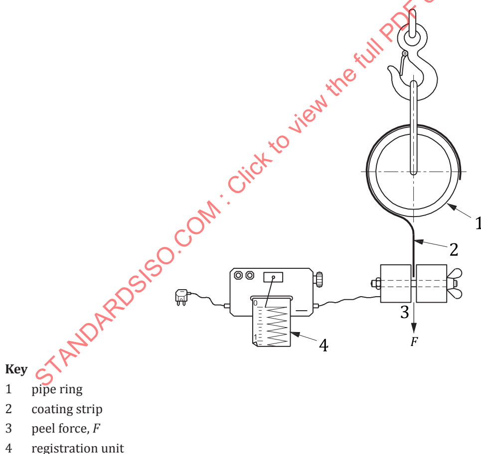
Figure C.1 — Peel strength test equipment for a small-diameter pipe
