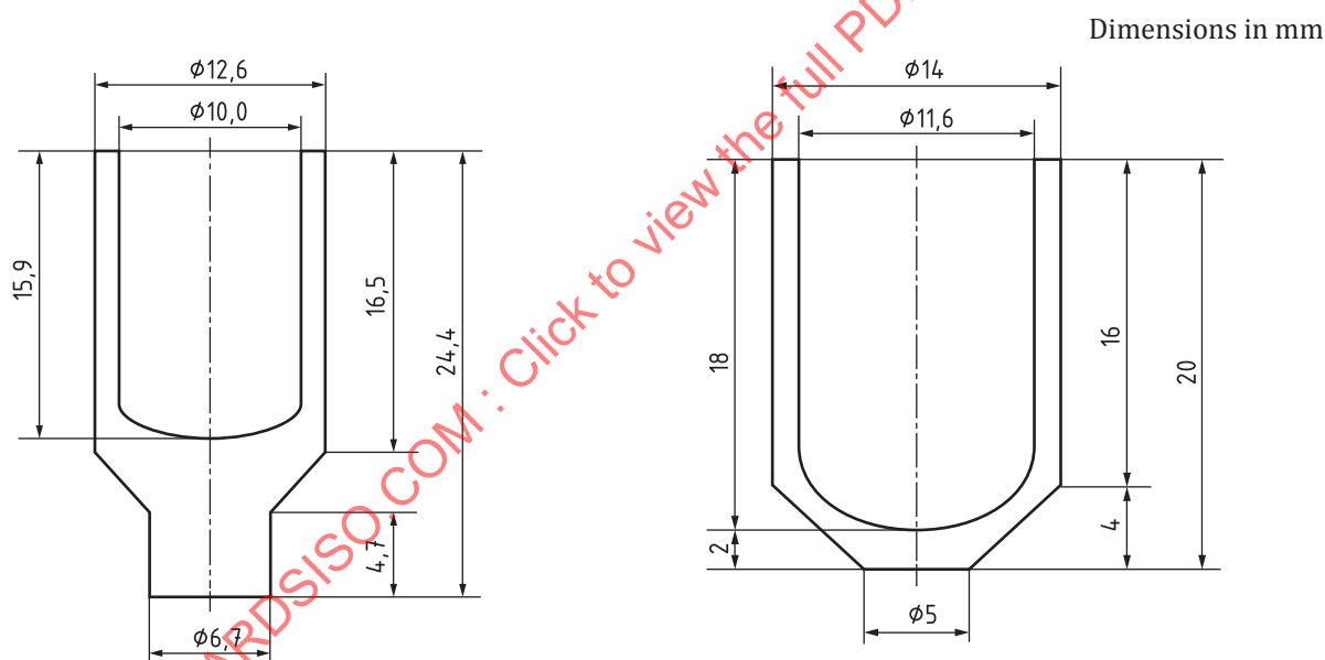
Figure 3 — Examples of a graphite crucible
