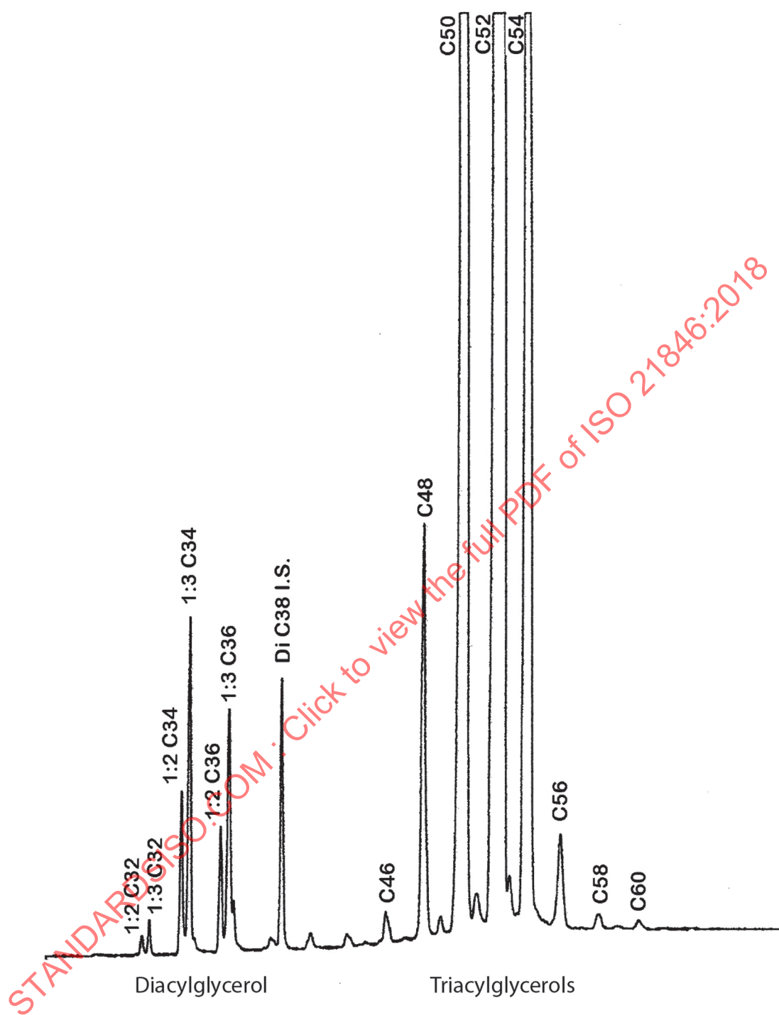
Figure A.2 — GLC trace of diacylglycerols and triacylglycerols of a palm olein sample
