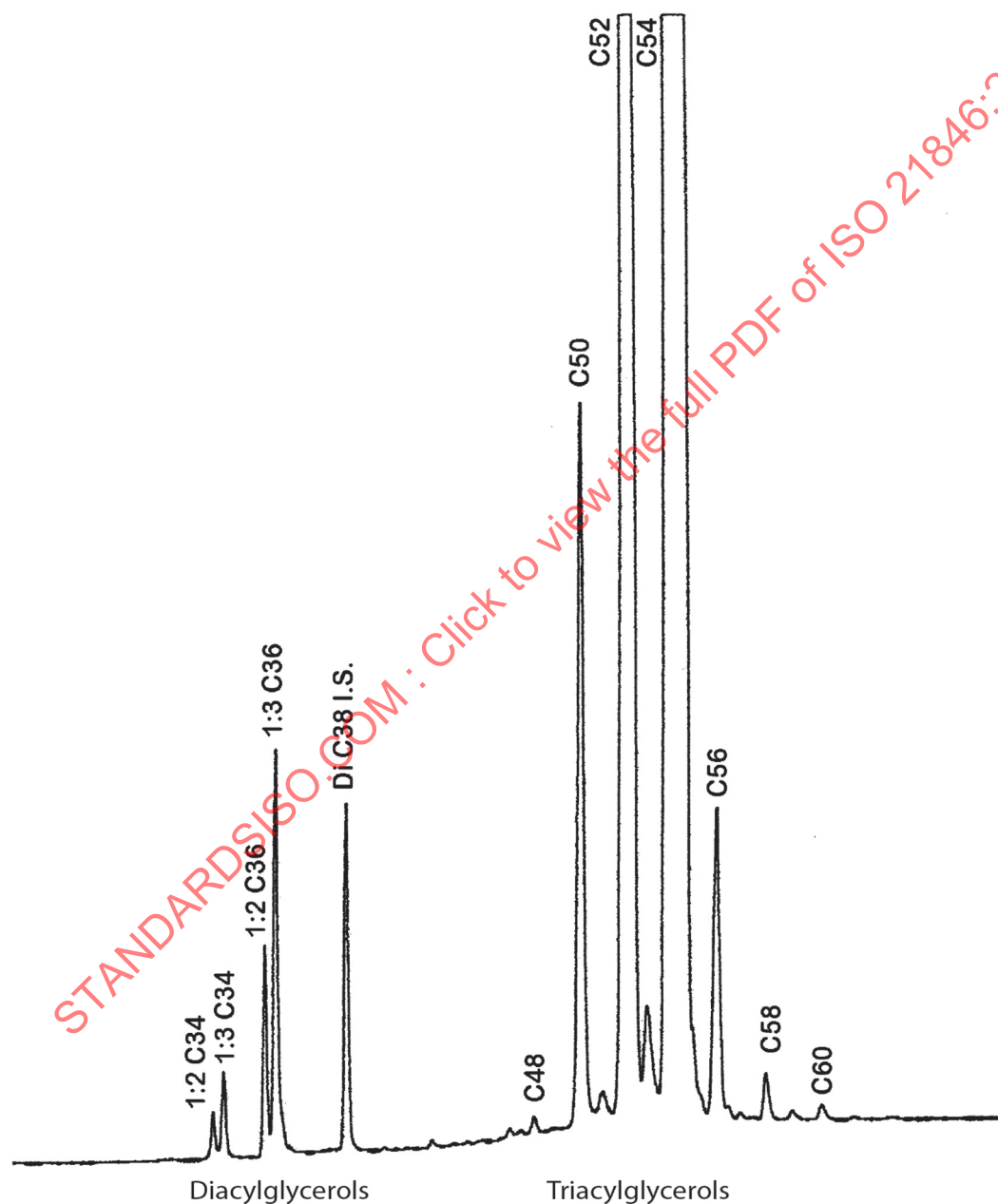
Figure A.1 — GLC trace of diacylglycerols and triacylglycerols of an olive oil sample
