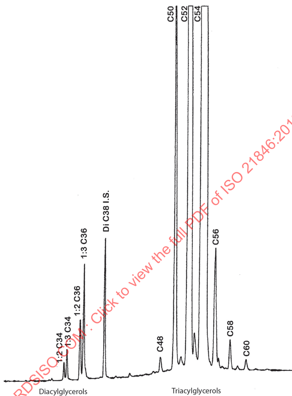
Figure A.4 — GLC trace of diacylglycerols and triacylglycerols of an olive oil mixed with palm olein and high oleic sunflower oil
