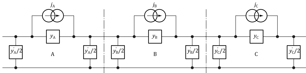
a) Equivalent-pi sections for a pipeline
