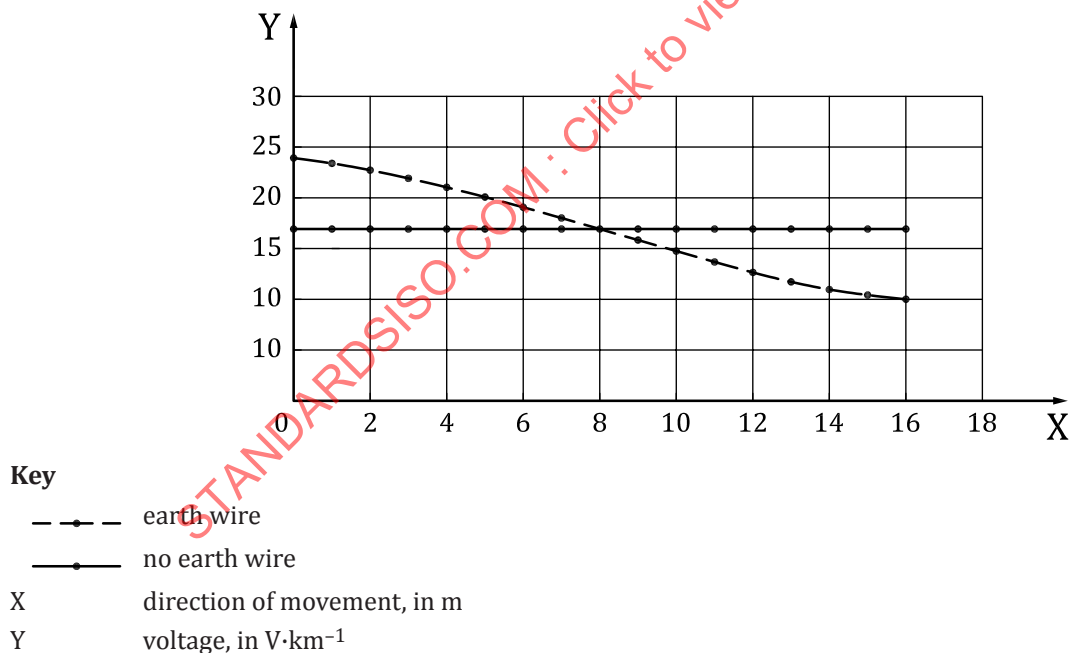
Figure F.1 — Difference in the calculated induced voltage on the pipe for the earth wire
