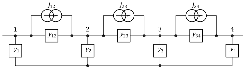
b) A nodal admittance network
