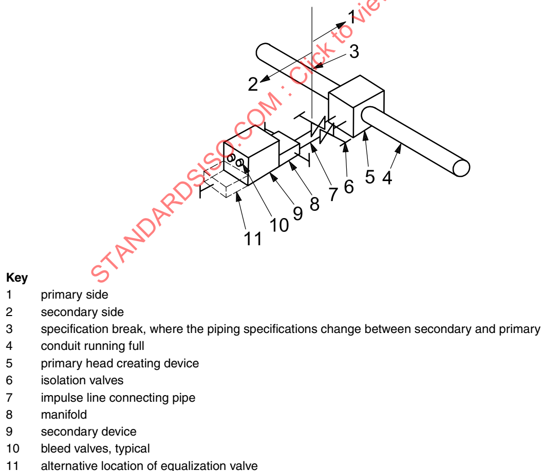
Figure 1 — Primary and secondary at same elevation, preferred installation
