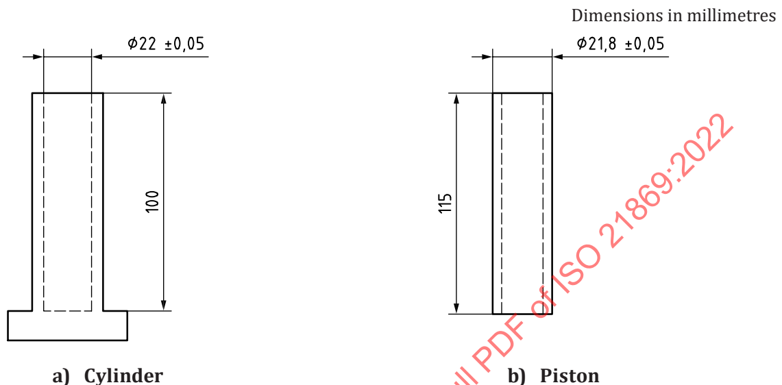
Figure 1 — Bulk density measuring apparatus
