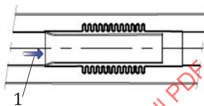
Figure C.1 — Sleeve covering the inner bellow ribs
