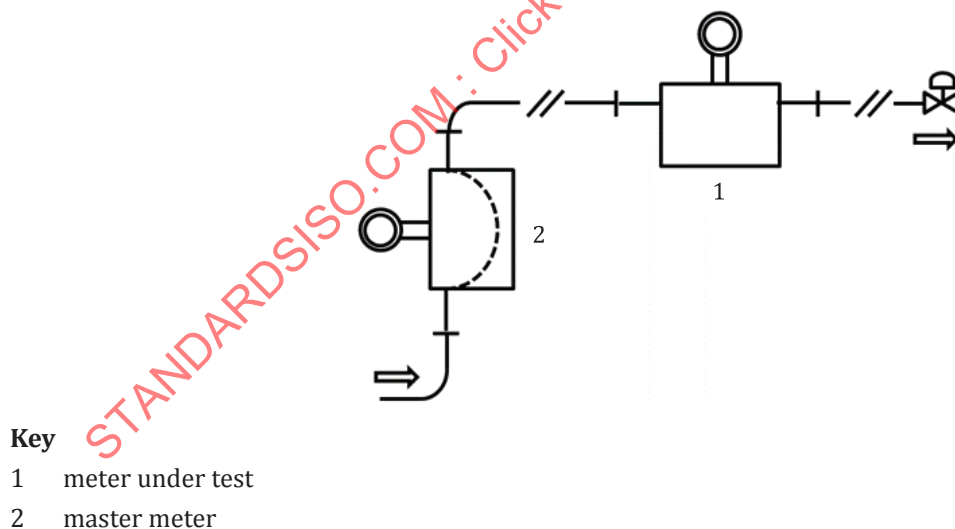
Figure 6 — Secondary flow standard master meter
