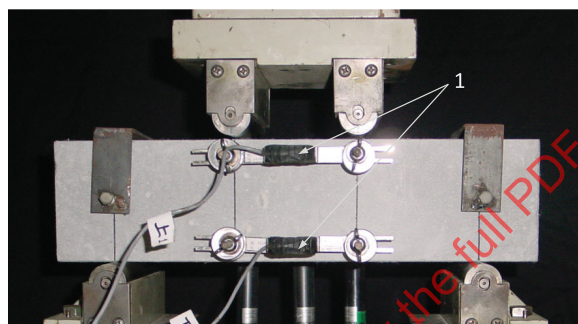
Figure 4 — Setup of LVDTs
