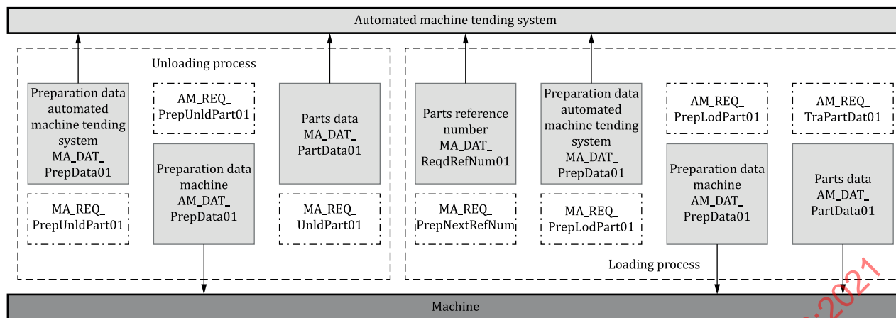
Figure 5 — Overview of possibilities for the use of preparation data and parts data
