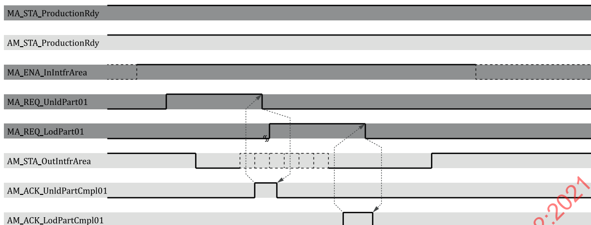
Figure C.3 — Interactions of all relevant signals at the control interface for a simple combined unloading and loading
