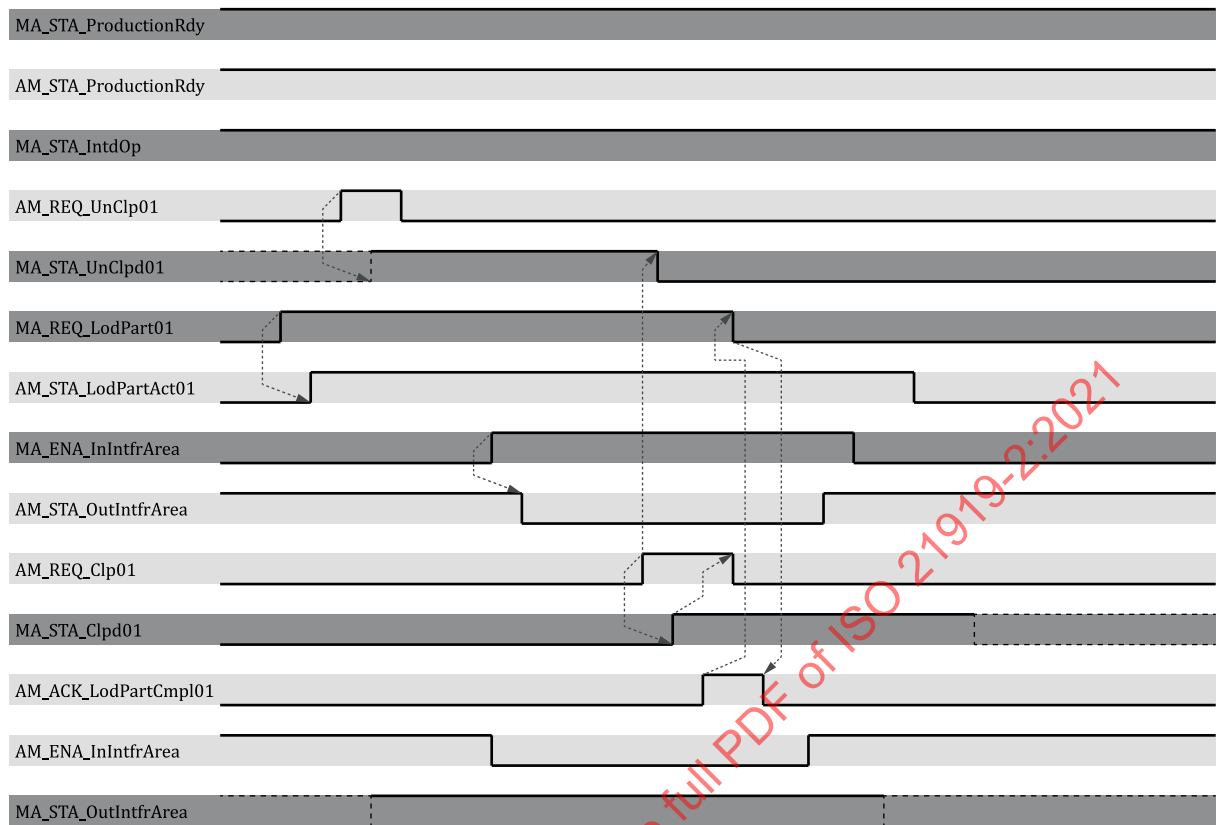
Figure C.7 — Interactions of all relevant signals at the control interface for loading with coherent transfer
