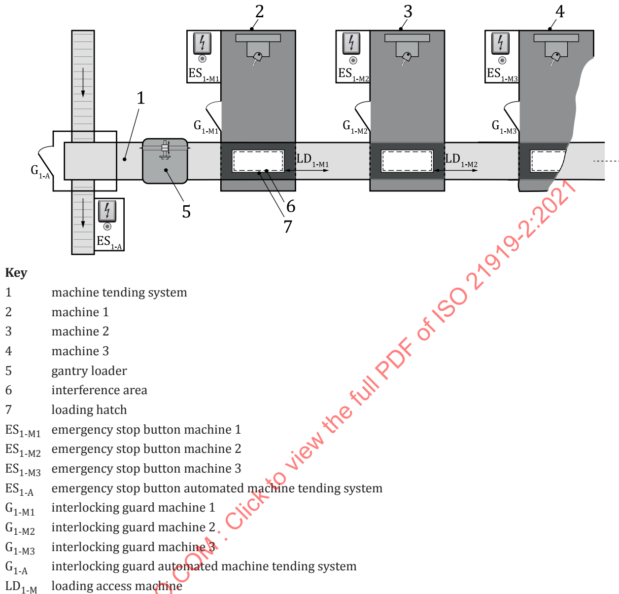
Figure B.5 — Loading of work space with loading access from above
