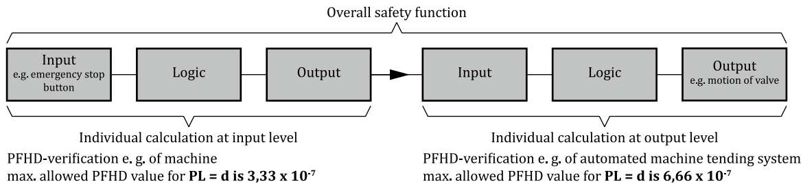
Figure 8 — Example on how to distribute PFHD values
