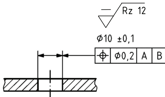
k) Graphical symbol readable from the bottom above geometrical tolerance indications away from the dimension line
