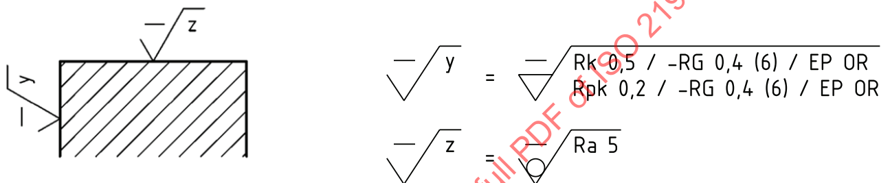
Figure 15 — Indication by the graphical symbol combined with a letter to specify identical and extensive requirements for several features
