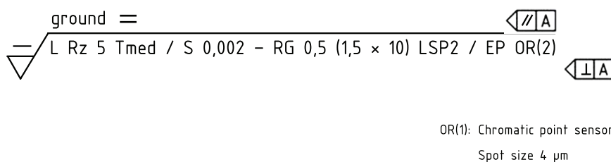
Figure D.5 — Indication for a section length R-parameter including all definable specification elements by using no default
