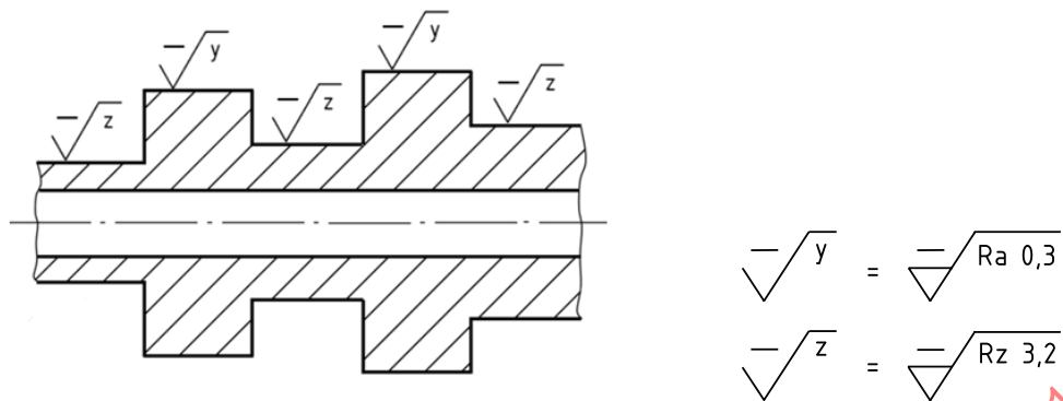
Figure 14 — Indication by the graphical symbol combined with a letter to specify identical requirements for several features
