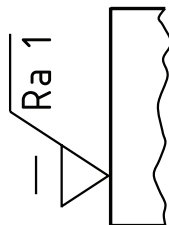
c) Graphical symbol readable from the right-hand side touches the surface
