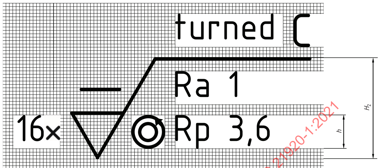
Figure A.3 — Proportions and dimensions
