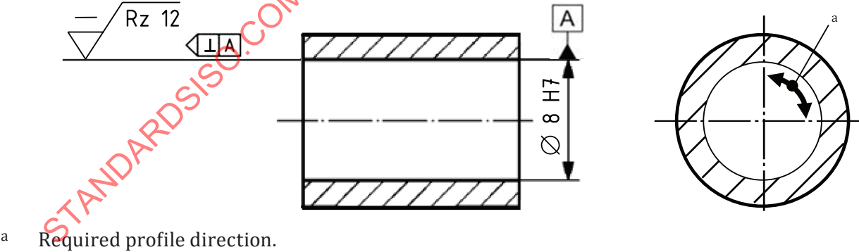
Figure 20 — Indication and interpretation of the specified profile direction by an intersection plane indicator in a 2D drawing
