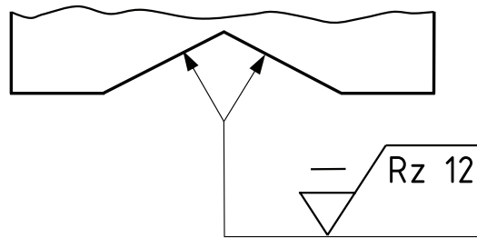
d) Graphical symbol readable from the bottom on a diverging leader line terminating in two arrowheads
