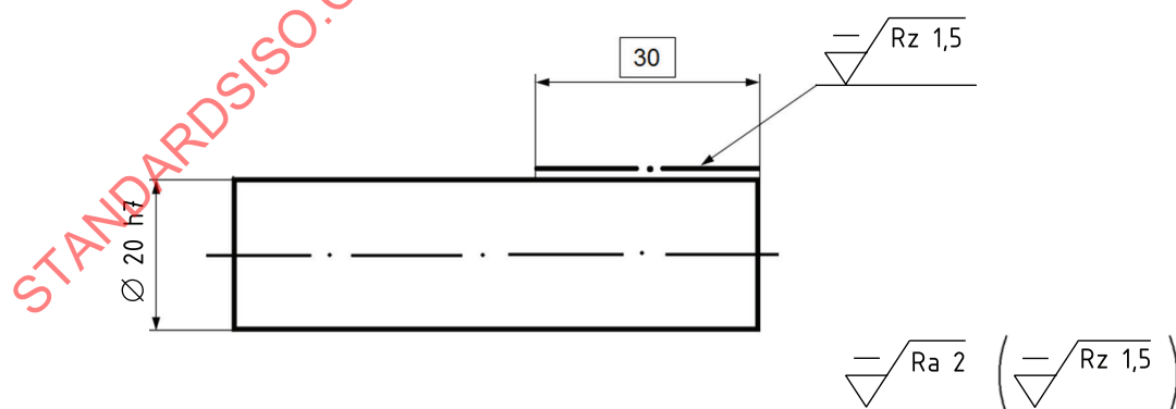
Figure 16 — Indication of a restricted part of a feature
