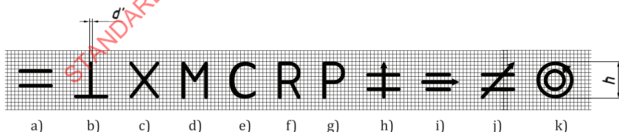
Figure A.2 — Proportions of the symbols
