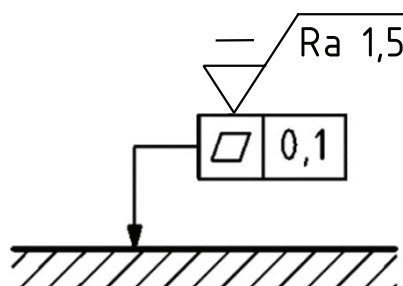
j) Graphical symbol readable from the bottom on the tolerance frame of a form, orientation, location or run-out requirement
