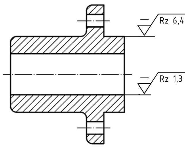
Figure 12 — Simplified indication followed by the graphical symbol
