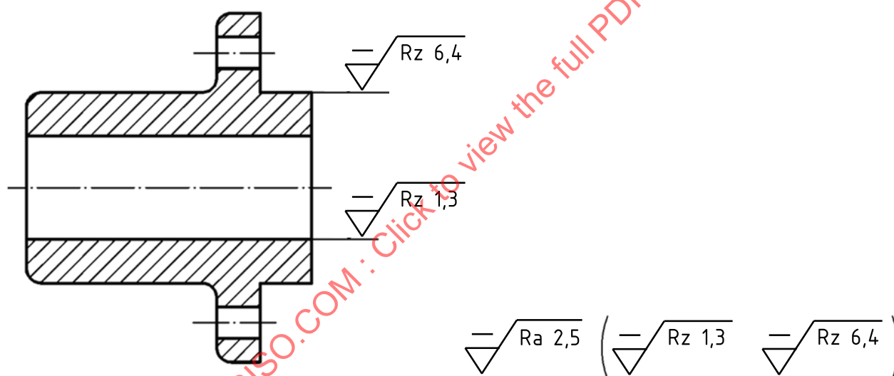
Figure 13 — Simplified indication followed by all other explicitly indicated requirements
