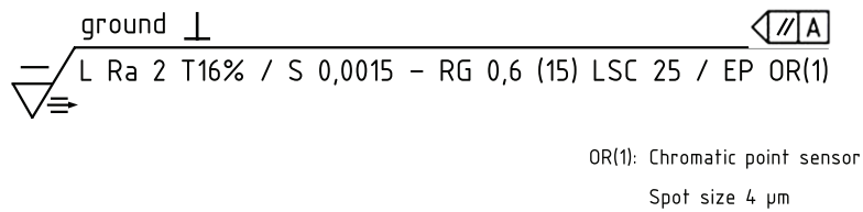
Figure D.4 — Indication for an evaluation length R-parameter including all definable specification elements by using no default
