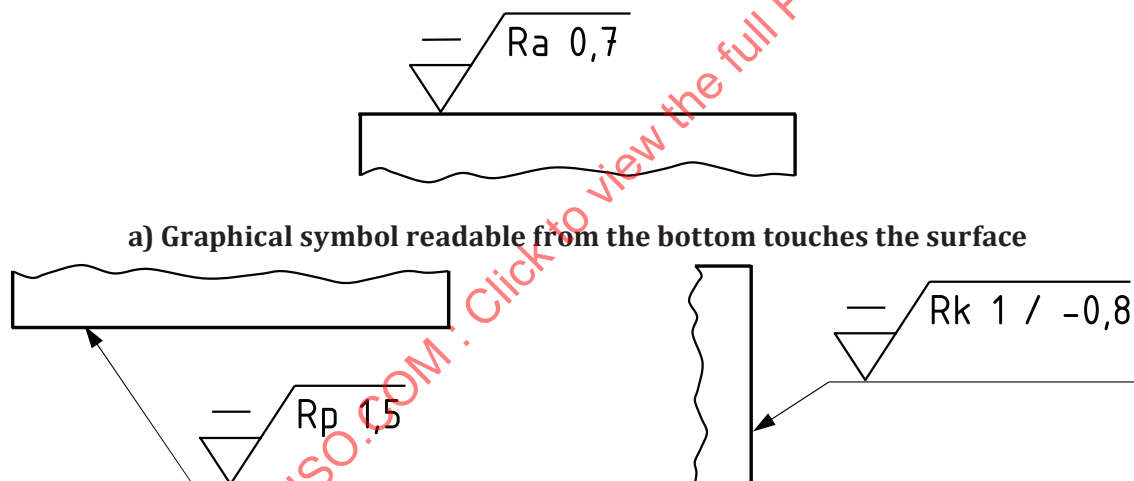
b) Graphical symbol readable from the bottom on a leader line terminating in an arrowhead
