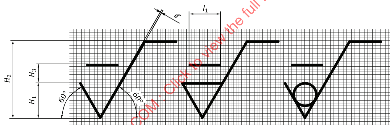
Figure A.1 — Proportions of the basic graphical symbol
